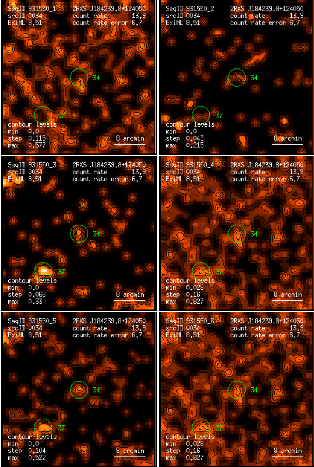
Figure 34: RASS 931550: detection 0034: band rate images, Gaussian filter: (1) PSPC channels 11 – 41, (2) 52 – 90, (3) 91 – 201, (4) 11 – 235, (5) 52 – 201, (6) 11 – 201. Broad band rates in counts/ks. Band rate contour levels in counts/ks/arcmin 2 .
