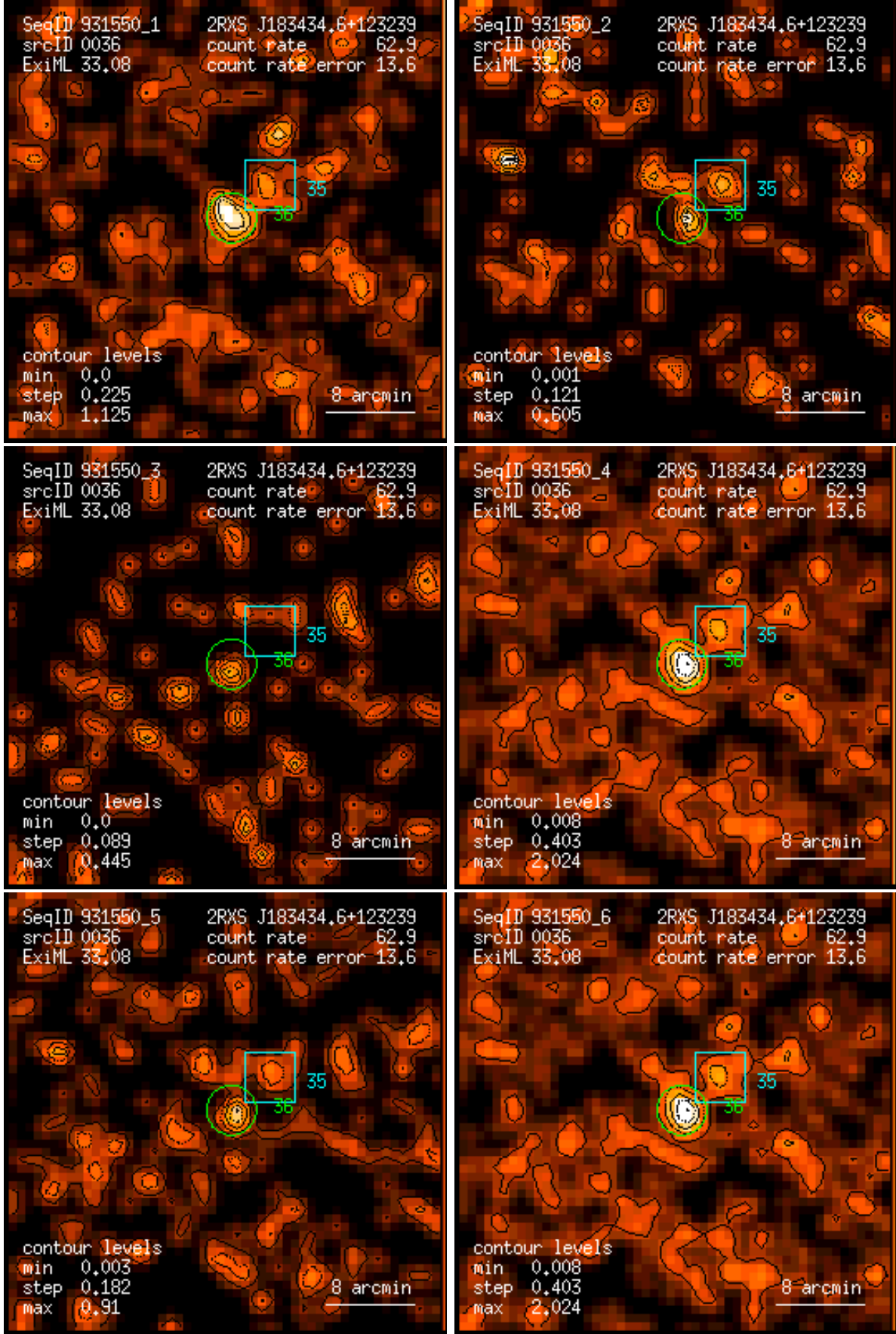
Figure 36: RASS 931550: detection 0036: band rate images, Gaussian filter: (1) PSPC channels 11 – 41, (2) 52 – 90, (3) 91 – 201, (4) 11 – 235, (5) 52 – 201, (6) 11 – 201. Broad band rates in counts/ks. Band rate contour levels in counts/ks/arcmin 2 .
