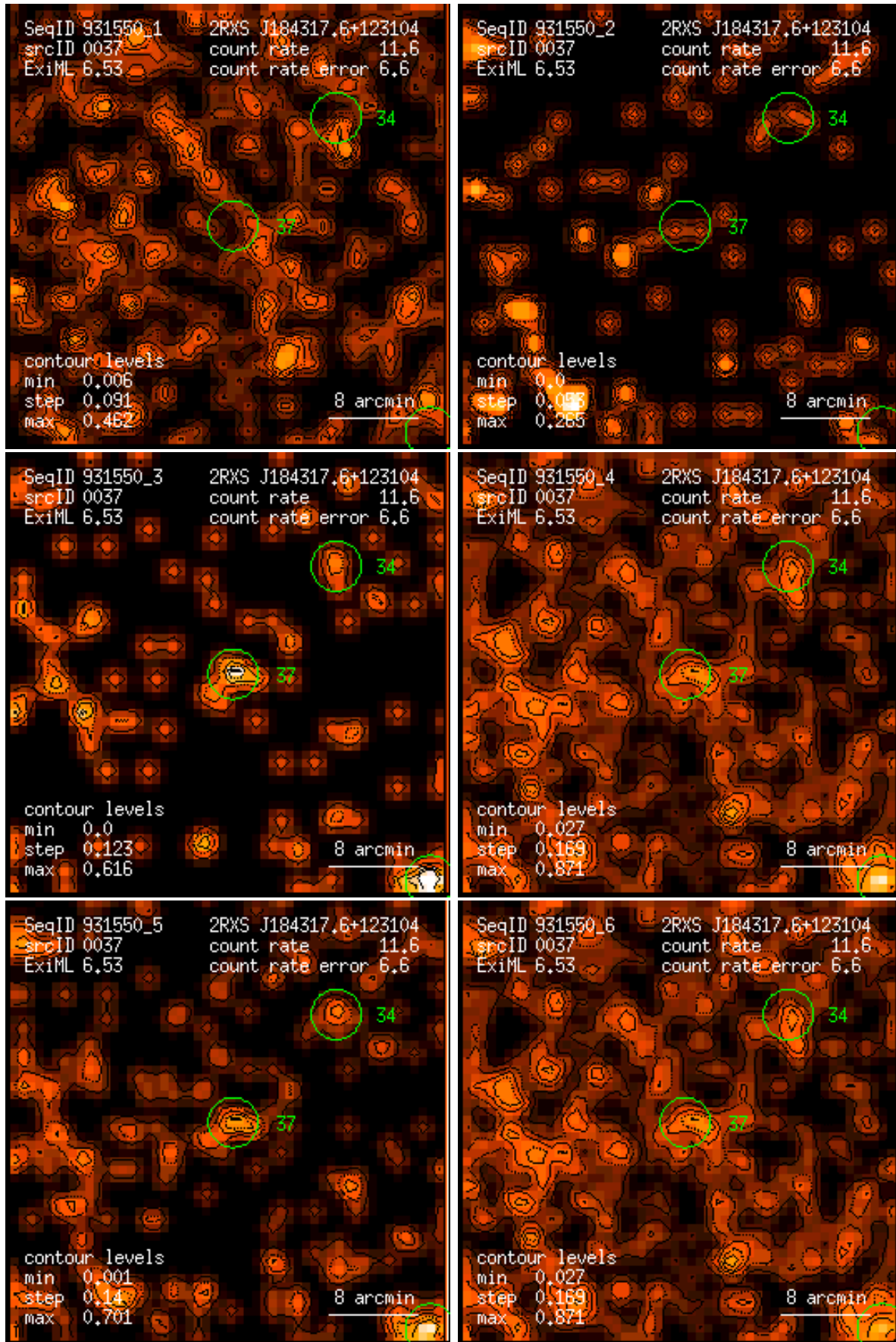
Figure 37: RASS 931550: detection 0037: band rate images, Gaussian filter: (1) PSPC channels 11 – 41, (2) 52 – 90, (3) 91 – 201, (4) 11 – 235, (5) 52 – 201, (6) 11 – 201. Broad band rates in counts/ks. Band rate contour levels in counts/ks/arcmin 2 .
