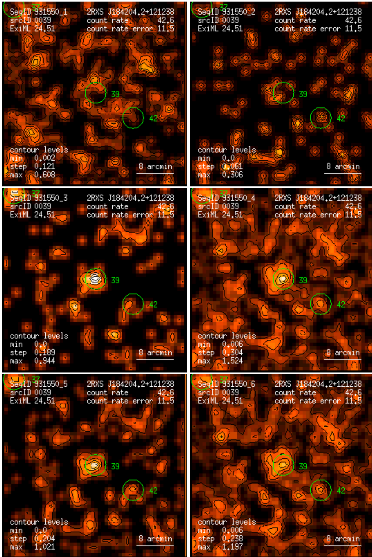
Figure 39: RASS 931550: detection 0039: band rate images, Gaussian filter: (1) PSPC channels 11 – 41, (2) 52 – 90, (3) 91 – 201, (4) 11 – 235, (5) 52 – 201, (6) 11 – 201. Broad band rates in counts/ks. Band rate contour levels in counts/ks/arcmin 2 .
