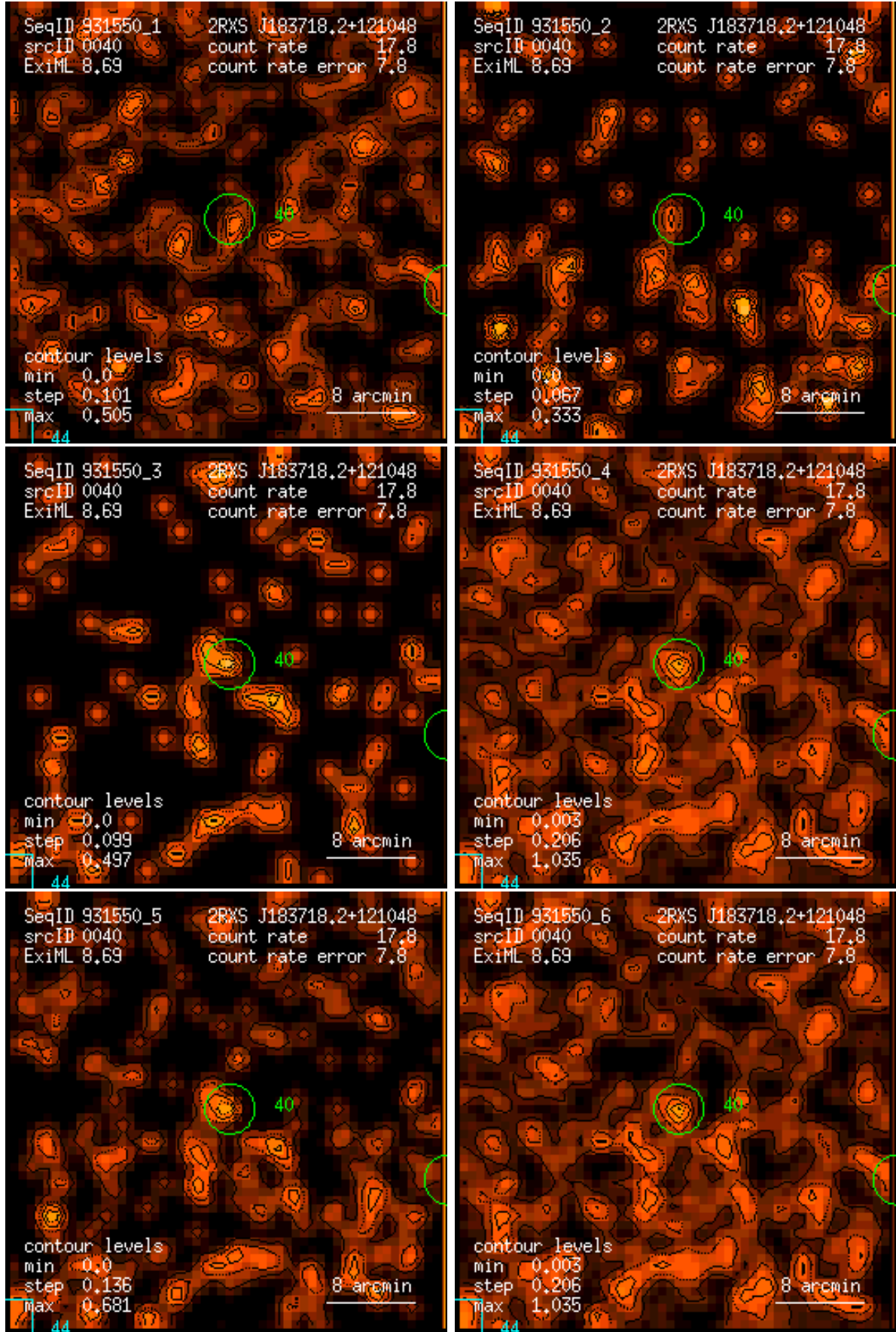
Figure 40: RASS 931550: detection 0040: band rate images, Gaussian filter: (1) PSPC channels 11 – 41, (2) 52 – 90, (3) 91 – 201, (4) 11 – 235, (5) 52 – 201, (6) 11 – 201. Broad band rates in counts/ks. Band rate contour levels in counts/ks/arcmin 2 .
