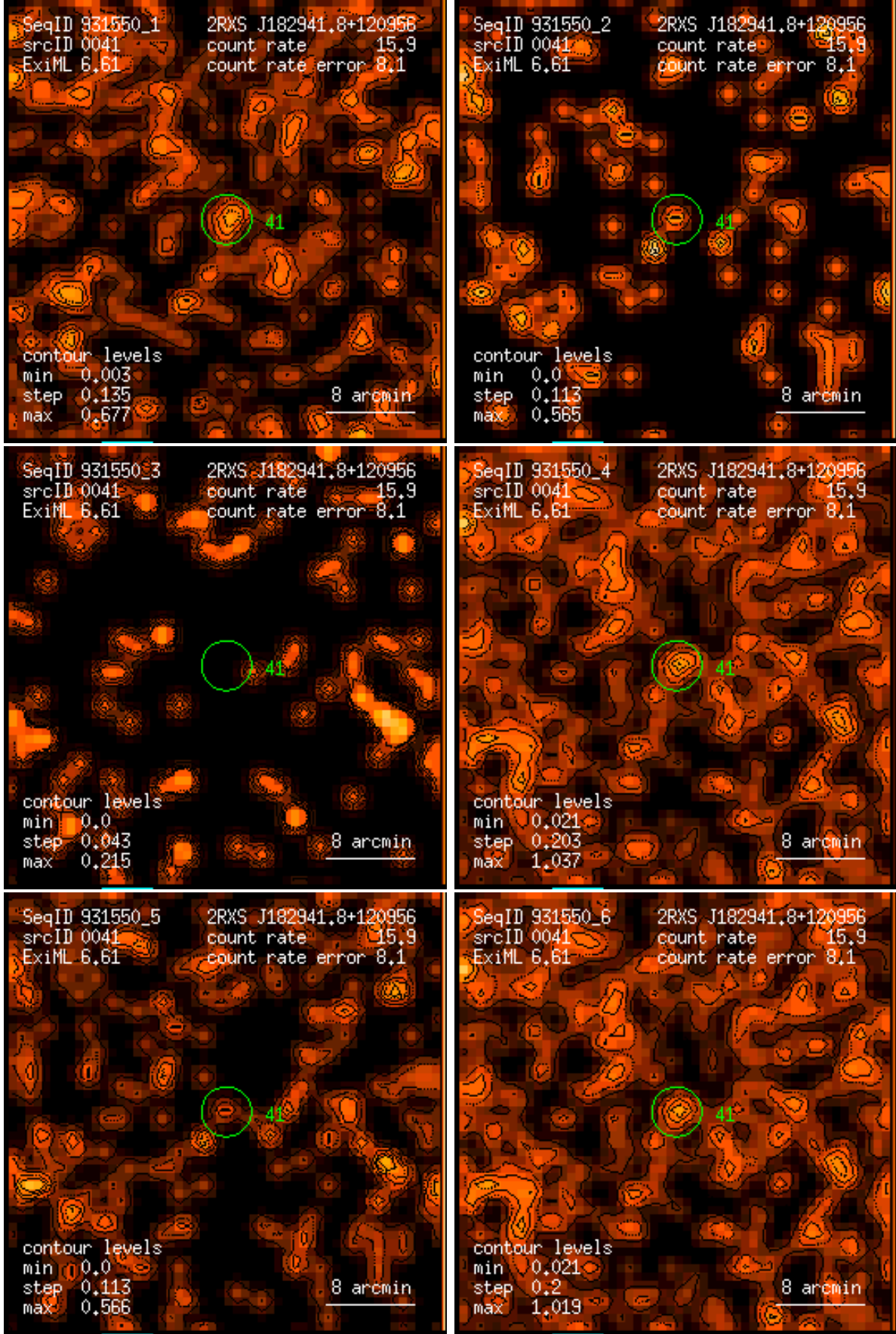
Figure 41: RASS 931550: detection 0041: band rate images, Gaussian filter: (1) PSPC channels 11 – 41, (2) 52 – 90, (3) 91 – 201, (4) 11 – 235, (5) 52 – 201, (6) 11 – 201. Broad band rates in counts/ks. Band rate contour levels in counts/ks/arcmin 2 .
