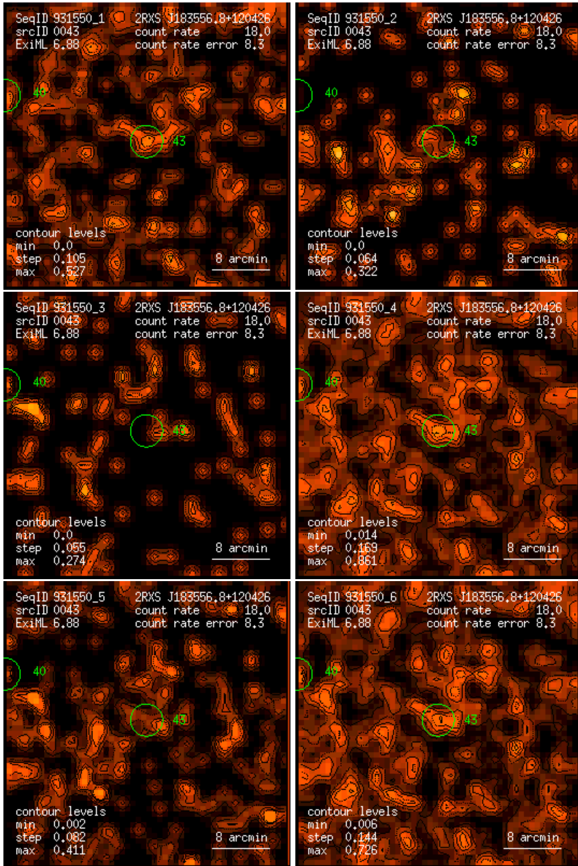
Figure 43: RASS 931550: detection 0043: band rate images, Gaussian filter: (1) PSPC channels 11 – 41, (2) 52 – 90, (3) 91 – 201, (4) 11 – 235, (5) 52 – 201, (6) 11 – 201. Broad band rates in counts/ks. Band rate contour levels in counts/ks/arcmin 2 .
