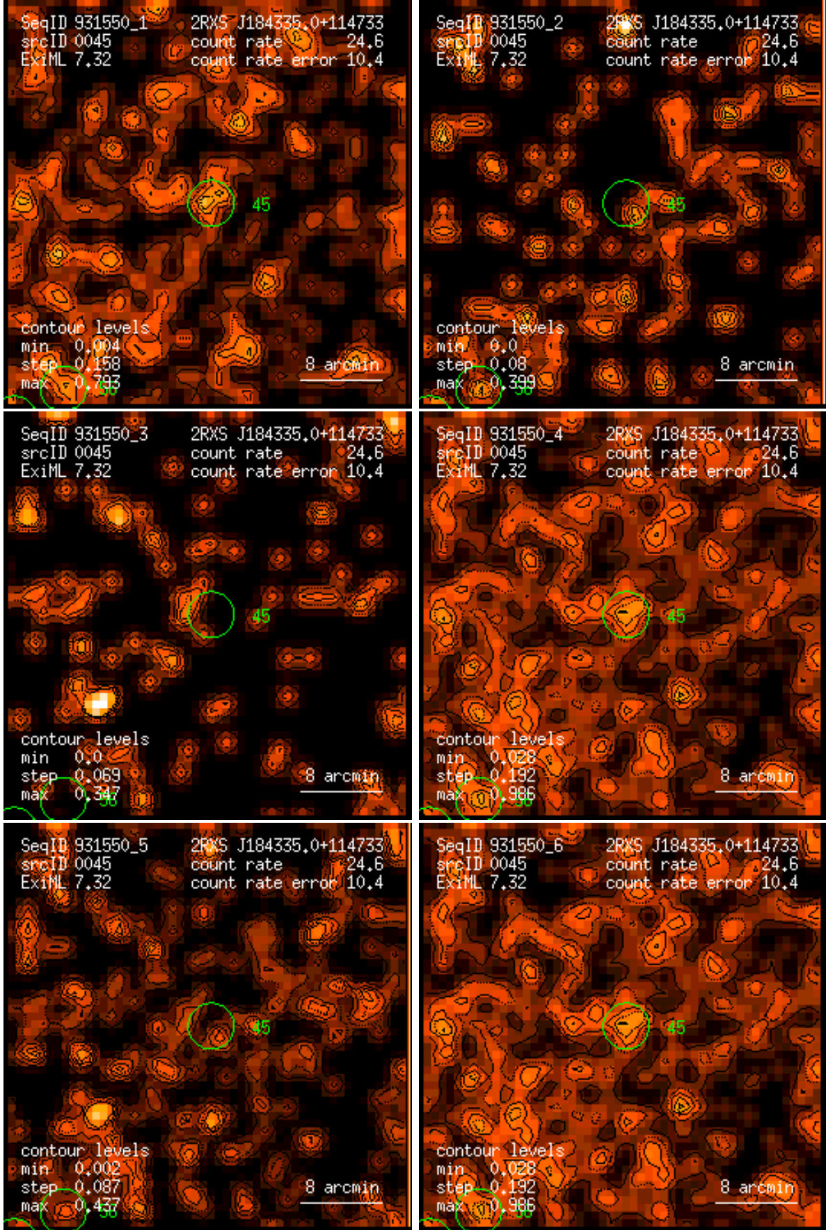
Figure 45: RASS 931550: detection 0045: band rate images, Gaussian filter: (1) PSPC channels 11 – 41, (2) 52 – 90, (3) 91 – 201, (4) 11 – 235, (5) 52 – 201, (6) 11 – 201. Broad band rates in counts/ks. Band rate contour levels in counts/ks/arcmin 2 .
