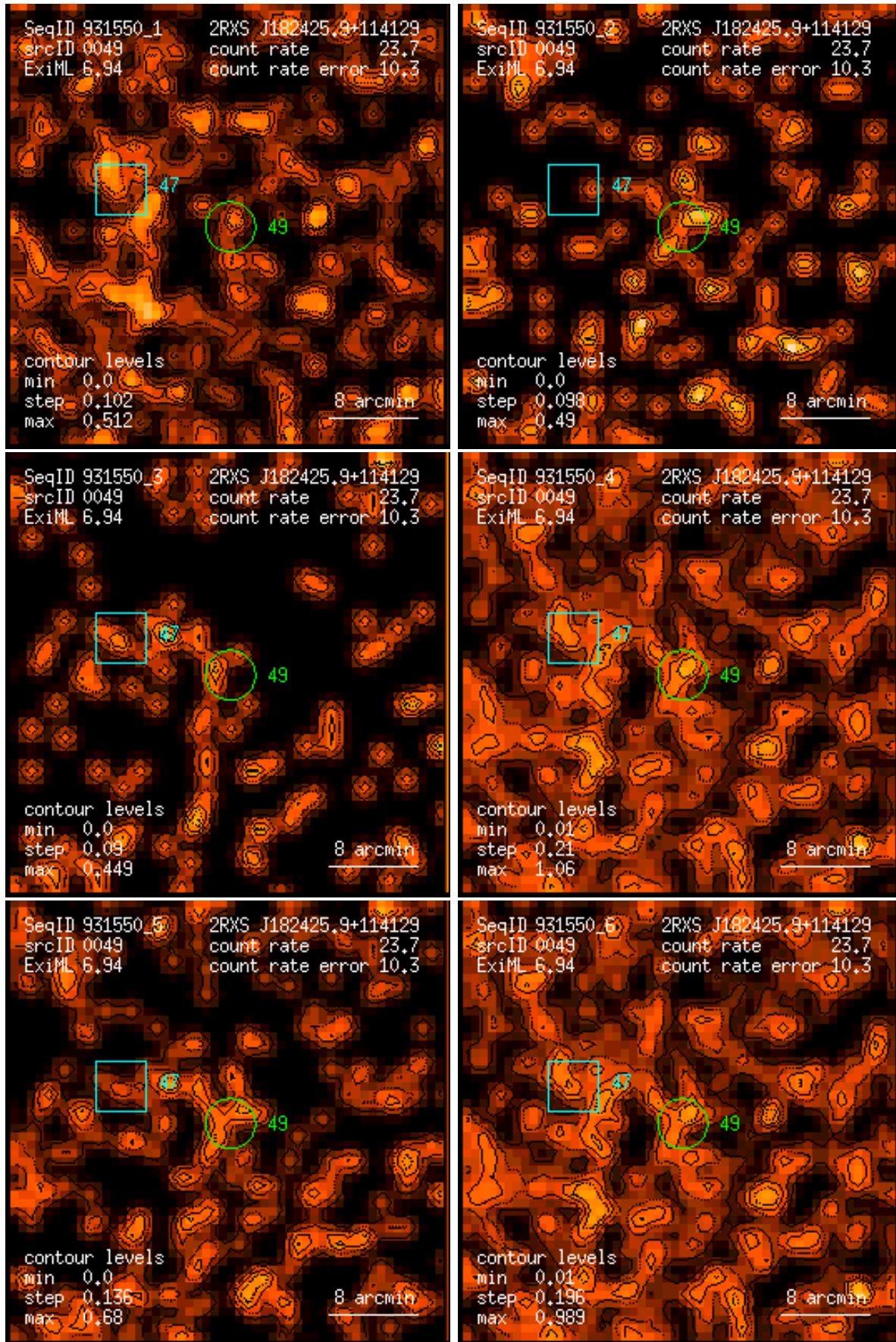
Figure 49: RASS 931550: detection 0049: band rate images, Gaussian filter: (1) PSPC channels 11 – 41, (2) 52 – 90, (3) 91 – 201, (4) 11 – 235, (5) 52 – 201, (6) 11 – 201. Broad band rates in counts/ks. Band rate contour levels in counts/ks/arcmin 2 .
