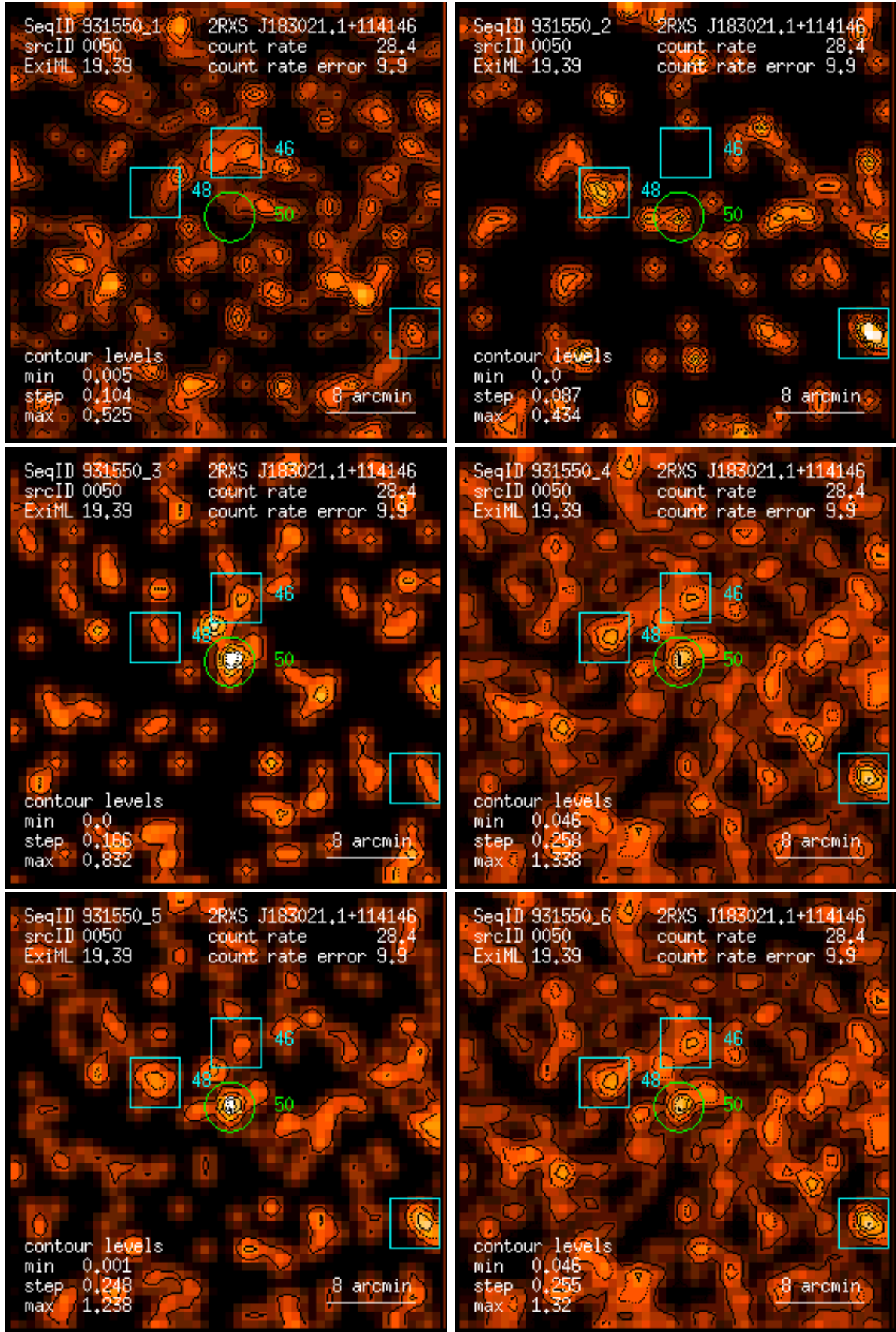
Figure 50: RASS 931550: detection 0050: band rate images, Gaussian filter: (1) PSPC channels 11 – 41, (2) 52 – 90, (3) 91 – 201, (4) 11 – 235, (5) 52 – 201, (6) 11 – 201. Broad band rates in counts/ks. Band rate contour levels in counts/ks/arcmin 2 .
