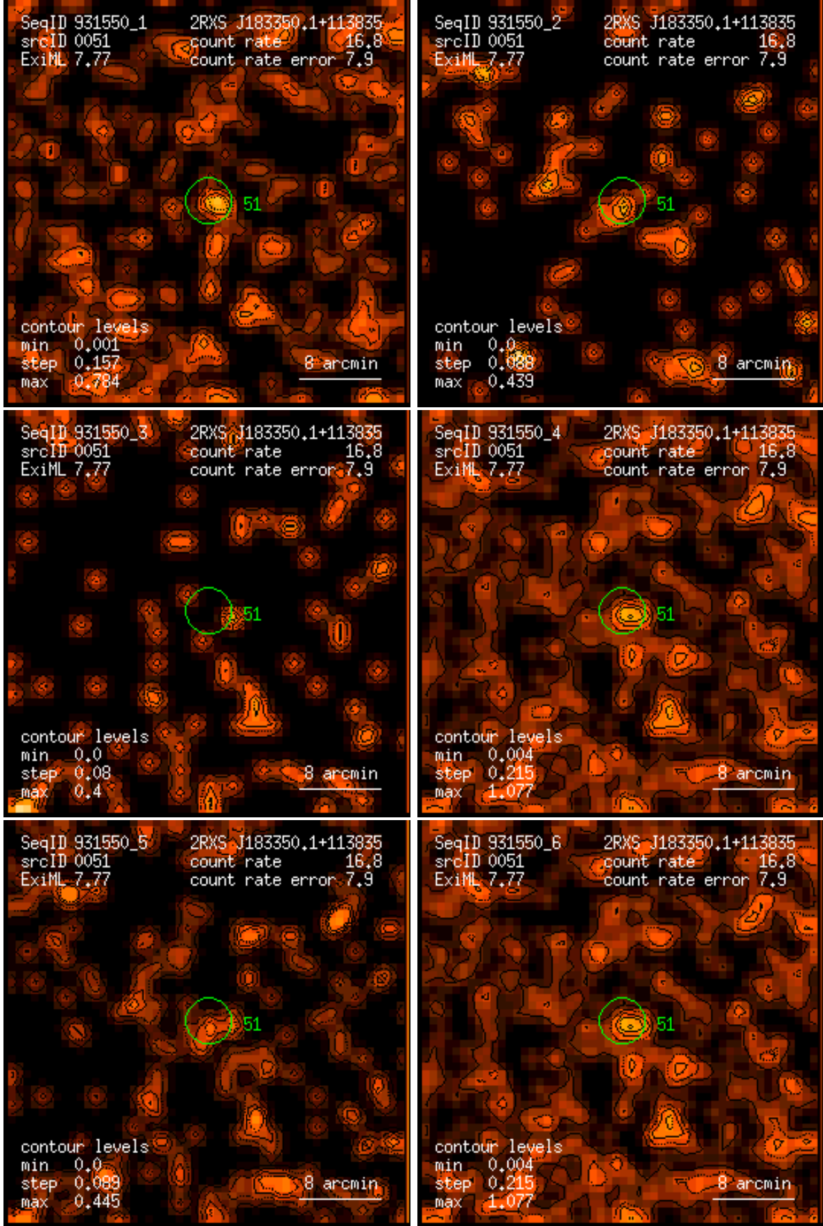
Figure 51: RASS 931550: detection 0051: band rate images, Gaussian filter: (1) PSPC channels 11 – 41, (2) 52 – 90, (3) 91 – 201, (4) 11 – 235, (5) 52 – 201, (6) 11 – 201. Broad band rates in counts/ks. Band rate contour levels in counts/ks/arcmin 2 .
