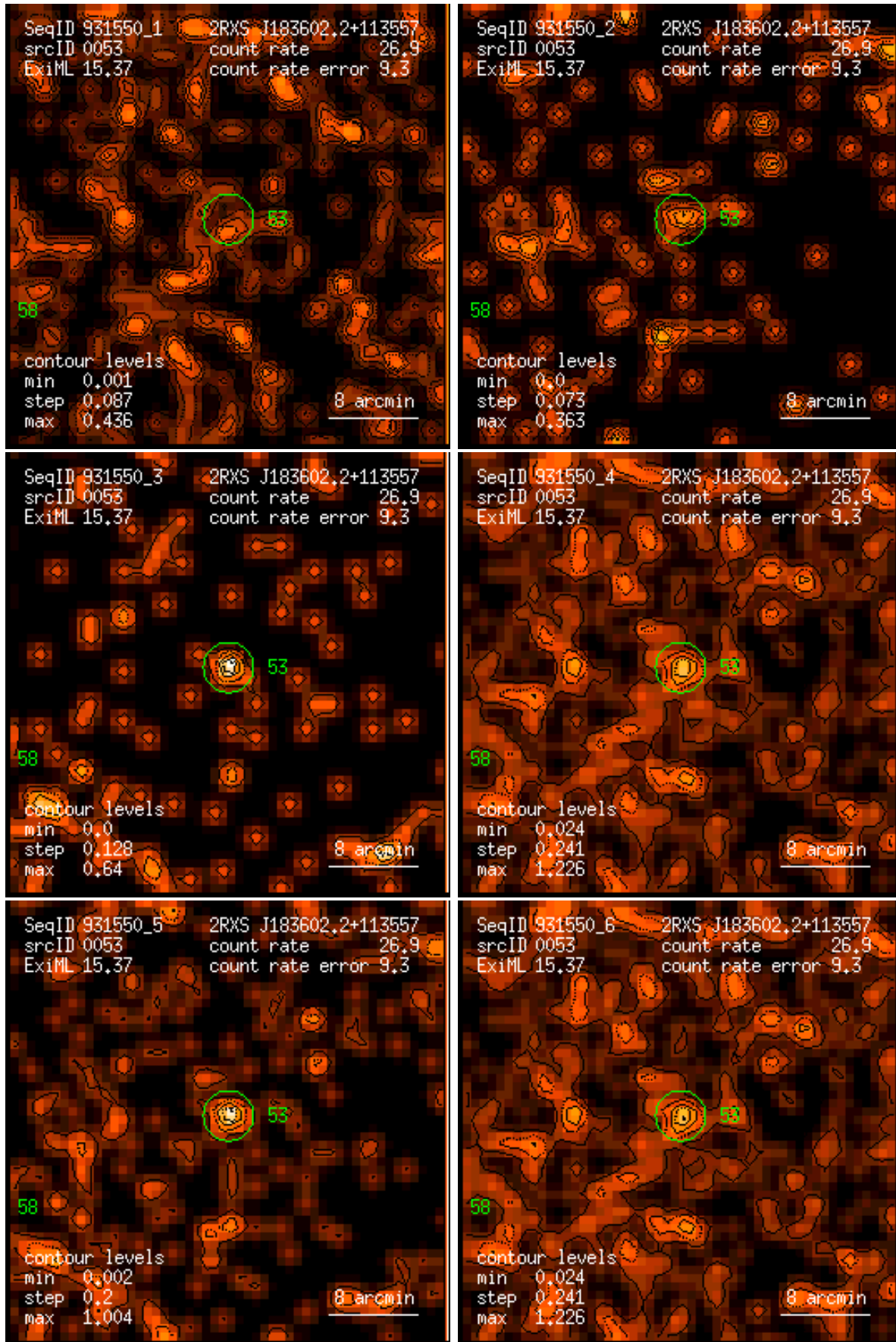
Figure 53: RASS 931550: detection 0053: band rate images, Gaussian filter: (1) PSPC channels 11 – 41, (2) 52 – 90, (3) 91 – 201, (4) 11 – 235, (5) 52 – 201, (6) 11 – 201. Broad band rates in counts/ks. Band rate contour levels in counts/ks/arcmin 2 .
