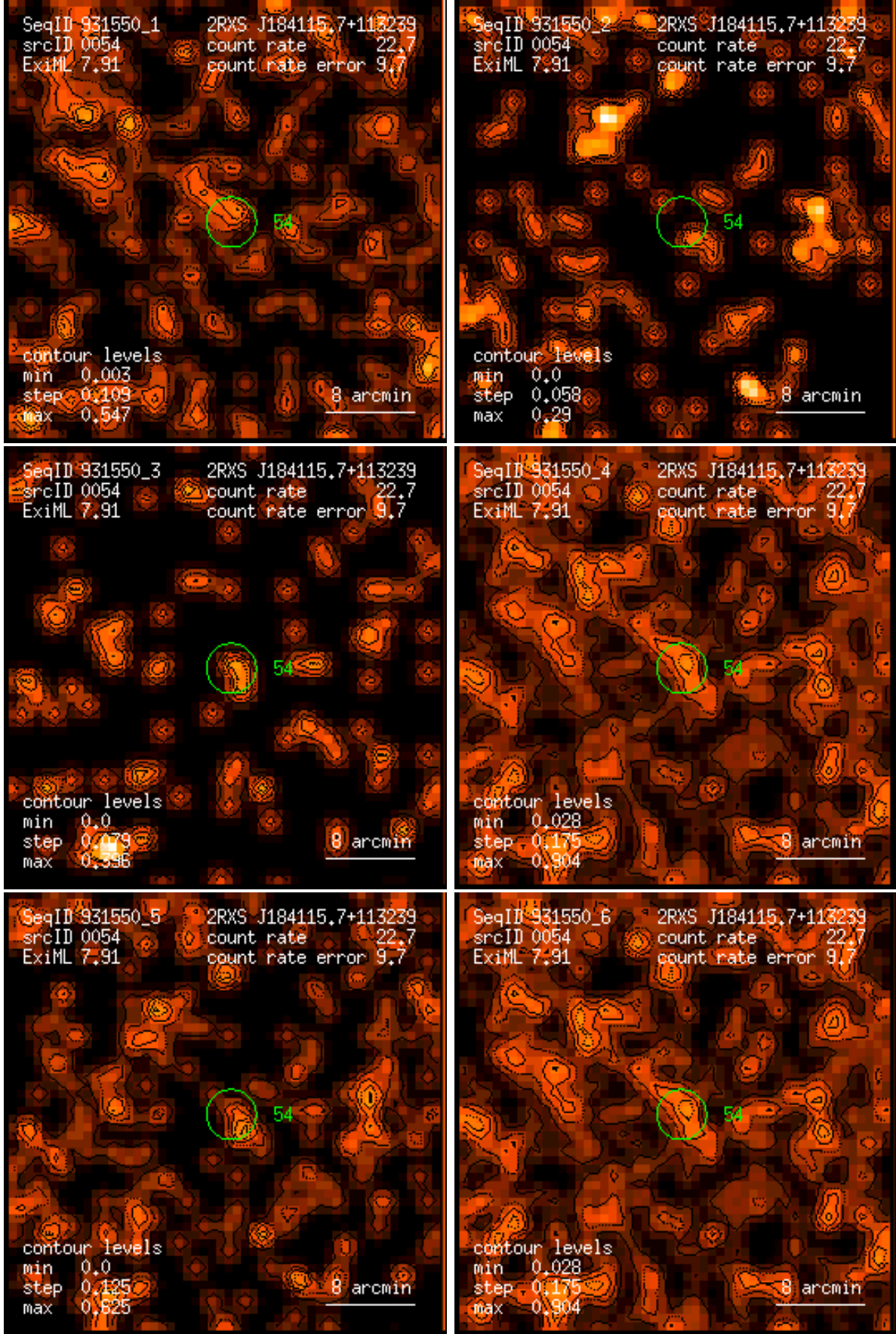
Figure 54: RASS 931550: detection 0054: band rate images, Gaussian filter: (1) PSPC channels 11 – 41, (2) 52 – 90, (3) 91 – 201, (4) 11 – 235, (5) 52 – 201, (6) 11 – 201. Broad band rates in counts/ks. Band rate contour levels in counts/ks/arcmin 2 .
