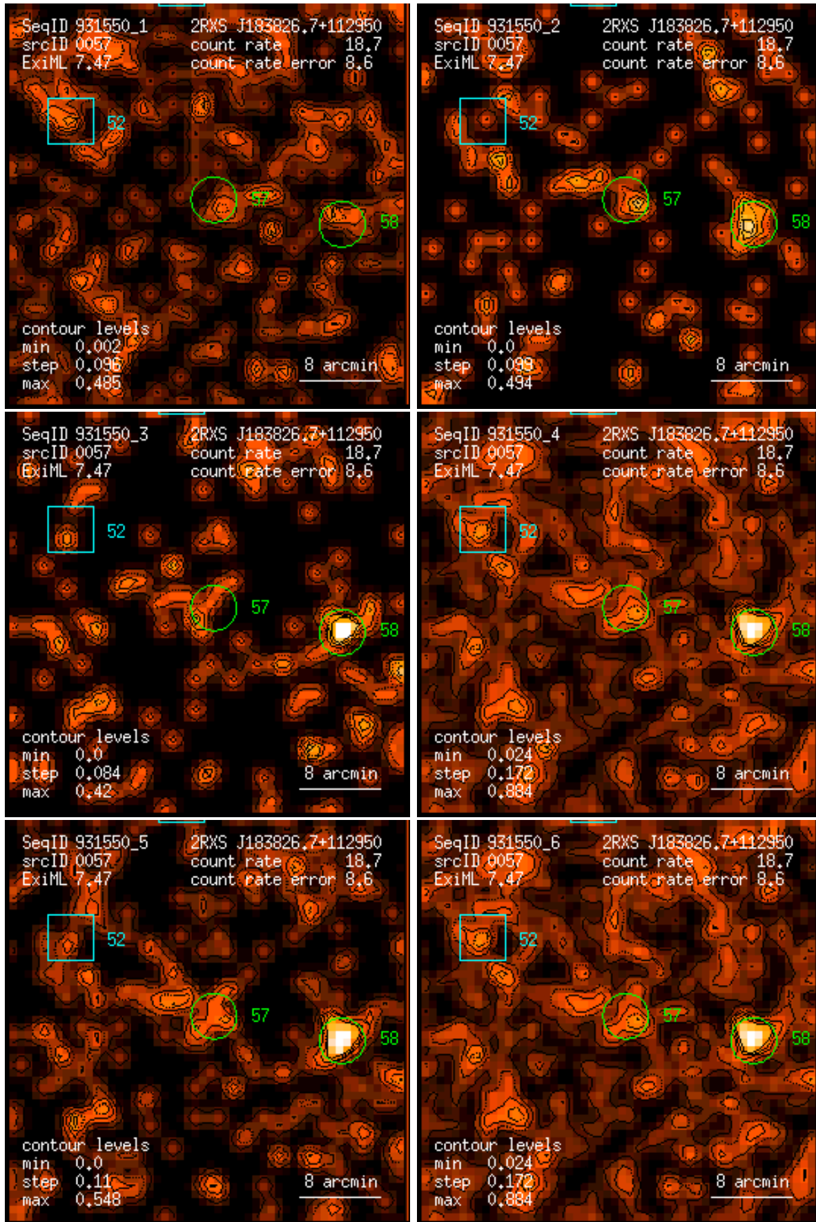
Figure 57: RASS 931550: detection 0057: band rate images, Gaussian filter: (1) PSPC channels 11 – 41, (2) 52 – 90, (3) 91 – 201, (4) 11 – 235, (5) 52 – 201, (6) 11 – 201. Broad band rates in counts/ks. Band rate contour levels in counts/ks/arcmin 2 .
