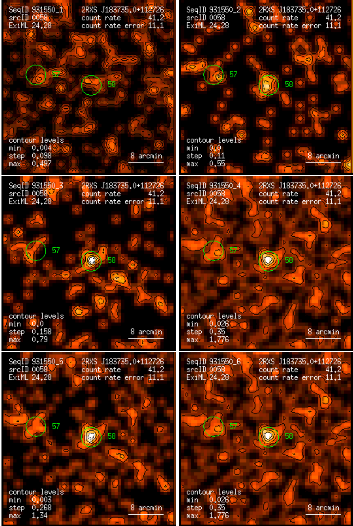
Figure 58: RASS 931550: detection 0058: band rate images, Gaussian filter: (1) PSPC channels 11 – 41, (2) 52 – 90, (3) 91 – 201, (4) 11 – 235, (5) 52 – 201, (6) 11 – 201. Broad band rates in counts/ks. Band rate contour levels in counts/ks/arcmin 2 .
