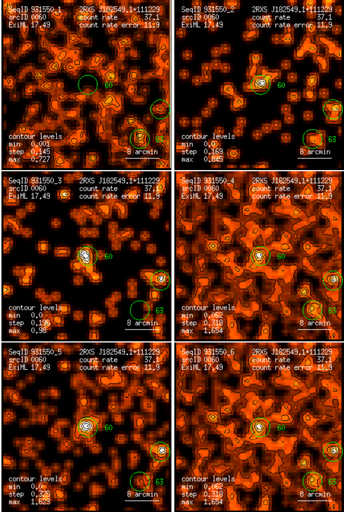
Figure 60: RASS 931550: detection 0060: band rate images, Gaussian filter: (1) PSPC channels 11 – 41, (2) 52 – 90, (3) 91 – 201, (4) 11 – 235, (5) 52 – 201, (6) 11 – 201. Broad band rates in counts/ks. Band rate contour levels in counts/ks/arcmin 2 .
