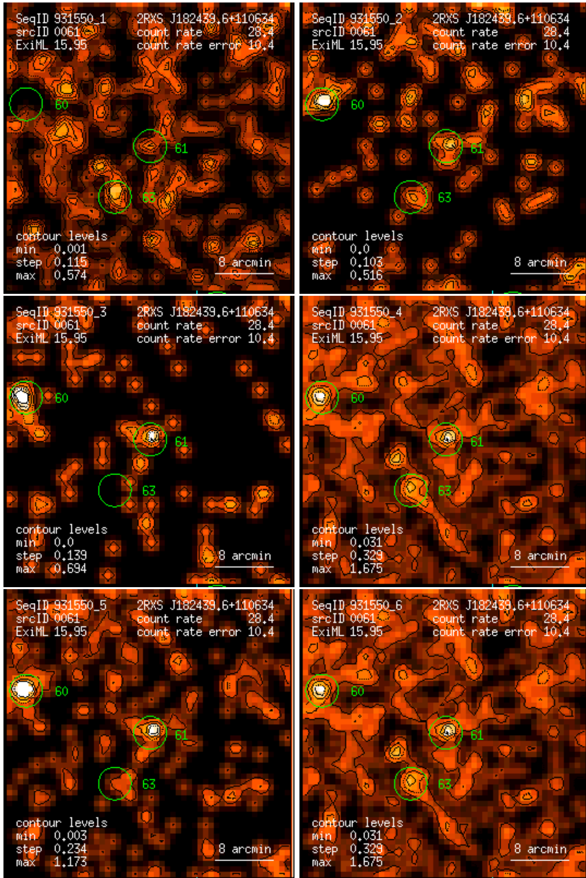
Figure 61: RASS 931550: detection 0061: band rate images, Gaussian filter: (1) PSPC channels 11 – 41, (2) 52 – 90, (3) 91 – 201, (4) 11 – 235, (5) 52 – 201, (6) 11 – 201. Broad band rates in counts/ks. Band rate contour levels in counts/ks/arcmin 2 .
