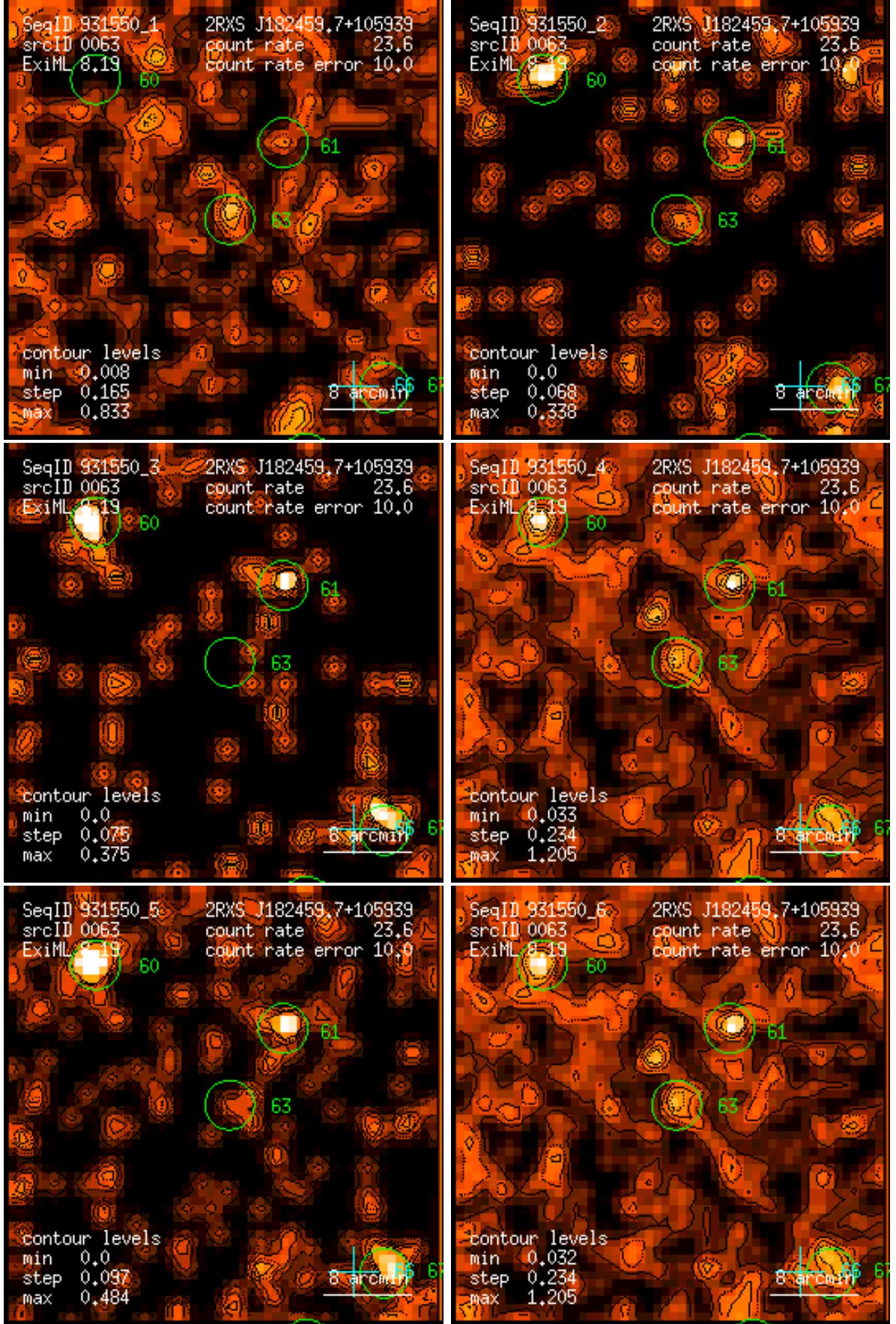
Figure 63: RASS 931550: detection 0063: band rate images, Gaussian filter: (1) PSPC channels 11 – 41, (2) 52 – 90, (3) 91 – 201, (4) 11 – 235, (5) 52 – 201, (6) 11 – 201. Broad band rates in counts/ks. Band rate contour levels in counts/ks/arcmin 2 .
