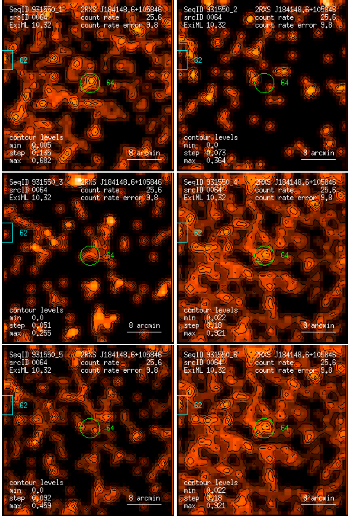
Figure 64: RASS 931550: detection 0064: band rate images, Gaussian filter: (1) PSPC channels 11 – 41, (2) 52 – 90, (3) 91 – 201, (4) 11 – 235, (5) 52 – 201, (6) 11 – 201. Broad band rates in counts/ks. Band rate contour levels in counts/ks/arcmin 2 .
