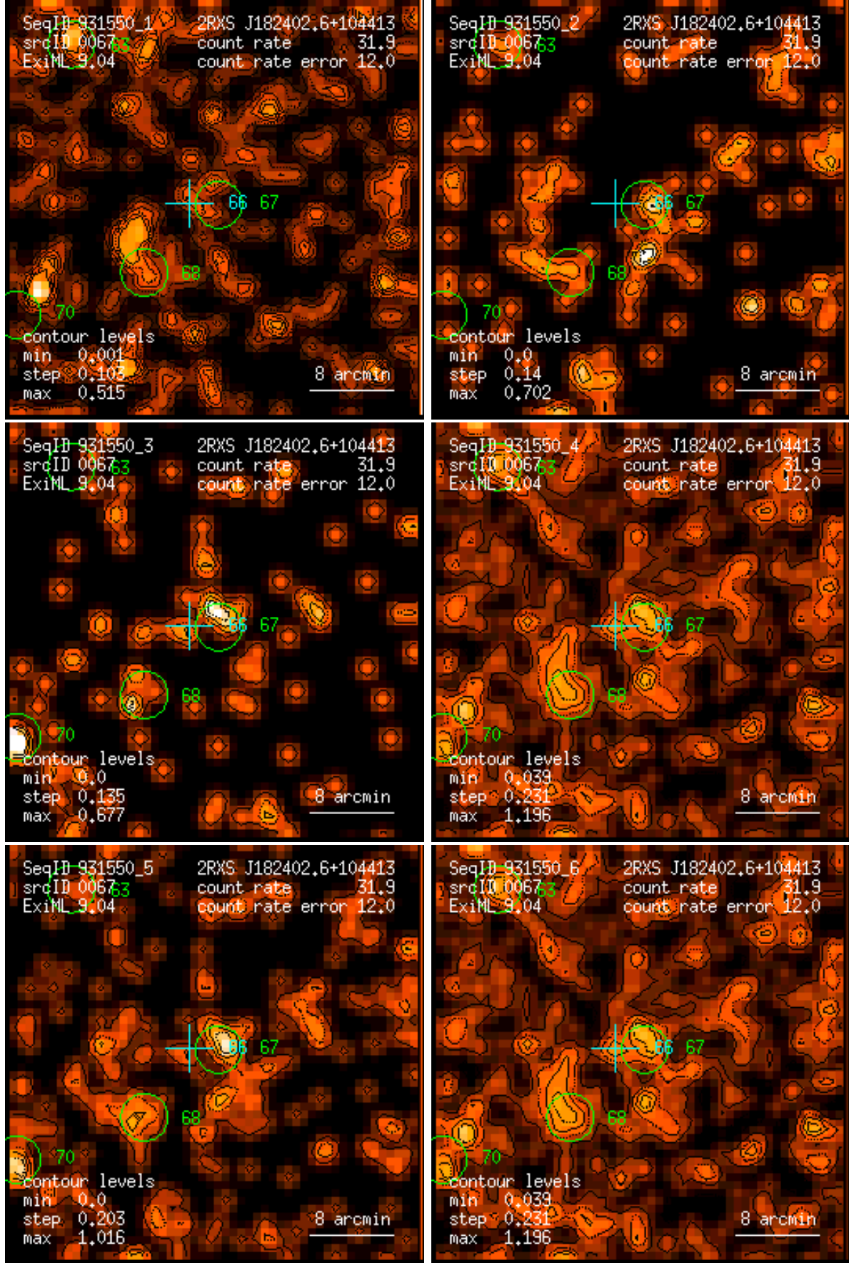
Figure 67: RASS 931550: detection 0067: band rate images, Gaussian filter: (1) PSPC channels 11 – 41, (2) 52 – 90, (3) 91 – 201, (4) 11 – 235, (5) 52 – 201, (6) 11 – 201. Broad band rates in counts/ks. Band rate contour levels in counts/ks/arcmin 2 .
