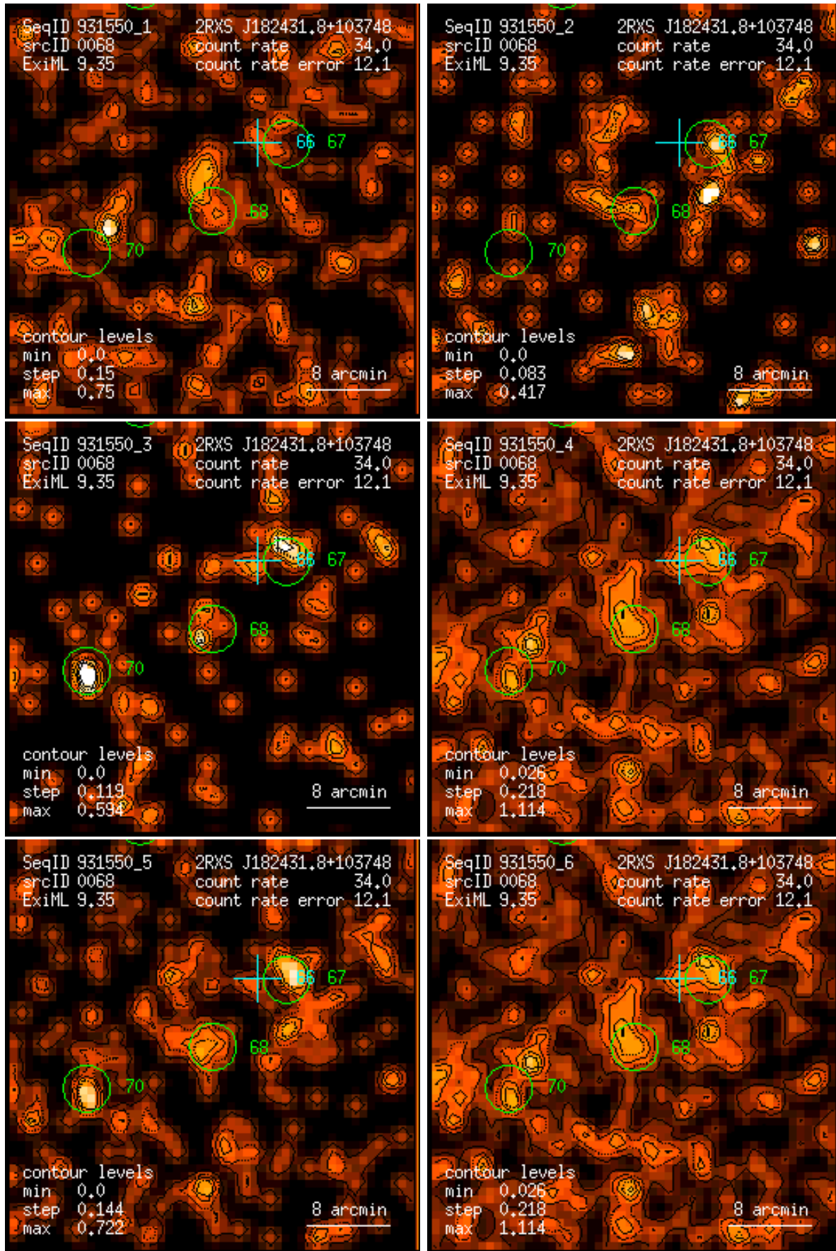
Figure 68: RASS 931550: detection 0068: band rate images, Gaussian filter: (1) PSPC channels 11 – 41, (2) 52 – 90, (3) 91 – 201, (4) 11 – 235, (5) 52 – 201, (6) 11 – 201. Broad band rates in counts/ks. Band rate contour levels in counts/ks/arcmin 2 .
