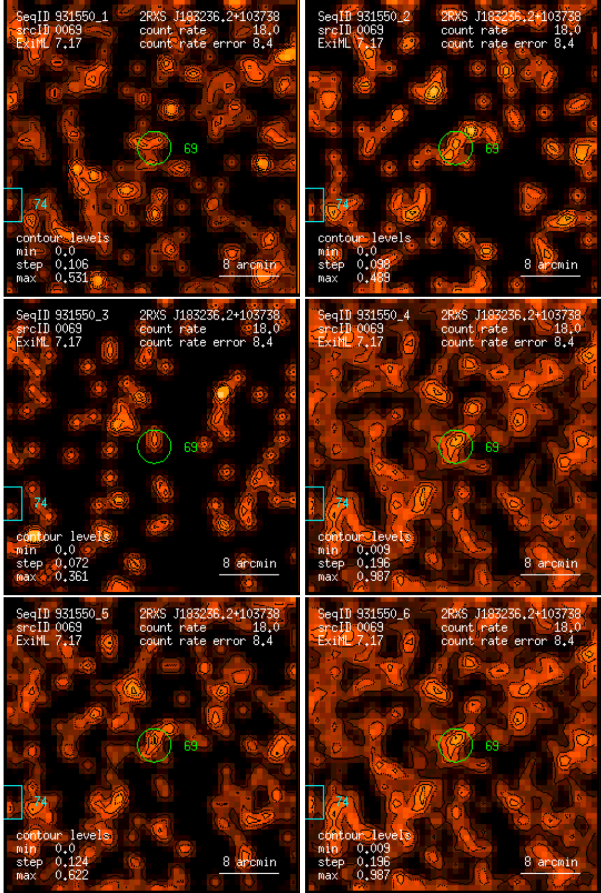
Figure 69: RASS 931550: detection 0069: band rate images, Gaussian filter: (1) PSPC channels 11 – 41, (2) 52 – 90, (3) 91 – 201, (4) 11 – 235, (5) 52 – 201, (6) 11 – 201. Broad band rates in counts/ks. Band rate contour levels in counts/ks/arcmin 2 .
