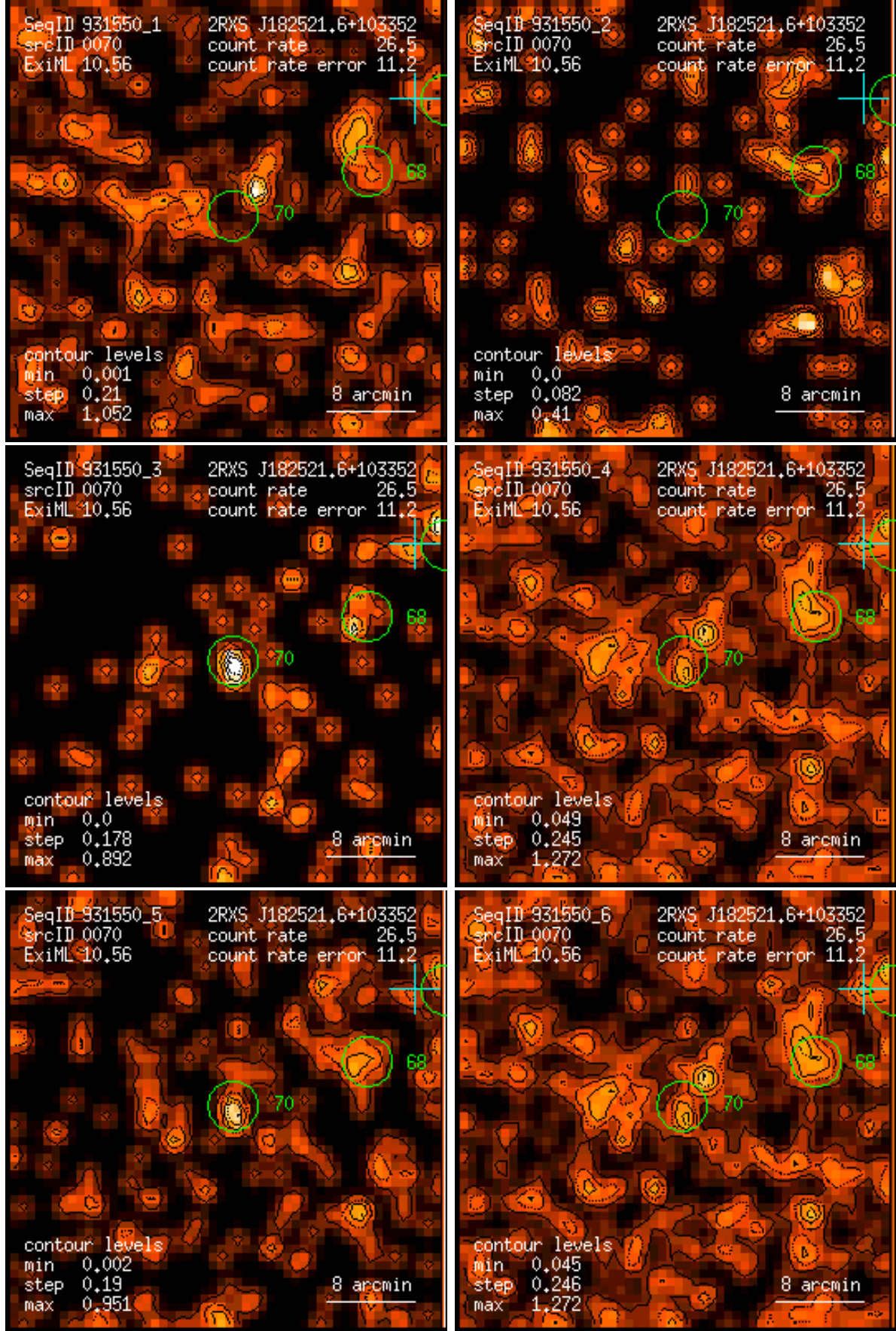
Figure 70: RASS 931550: detection 0070: band rate images, Gaussian filter: (1) PSPC channels 11 – 41, (2) 52 – 90, (3) 91 – 201, (4) 11 – 235, (5) 52 – 201, (6) 11 – 201. Broad band rates in counts/ks. Band rate contour levels in counts/ks/arcmin 2 .
