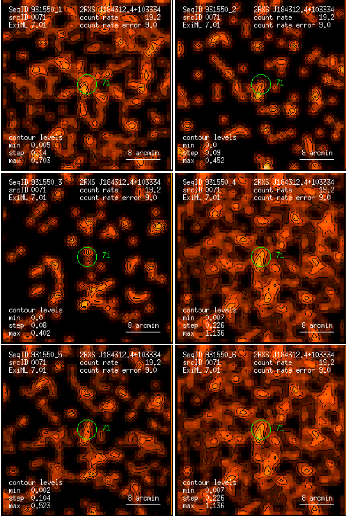
Figure 71: RASS 931550: detection 0071: band rate images, Gaussian filter: (1) PSPC channels 11 – 41, (2) 52 – 90, (3) 91 – 201, (4) 11 – 235, (5) 52 – 201, (6) 11 – 201. Broad band rates in counts/ks. Band rate contour levels in counts/ks/arcmin 2 .
