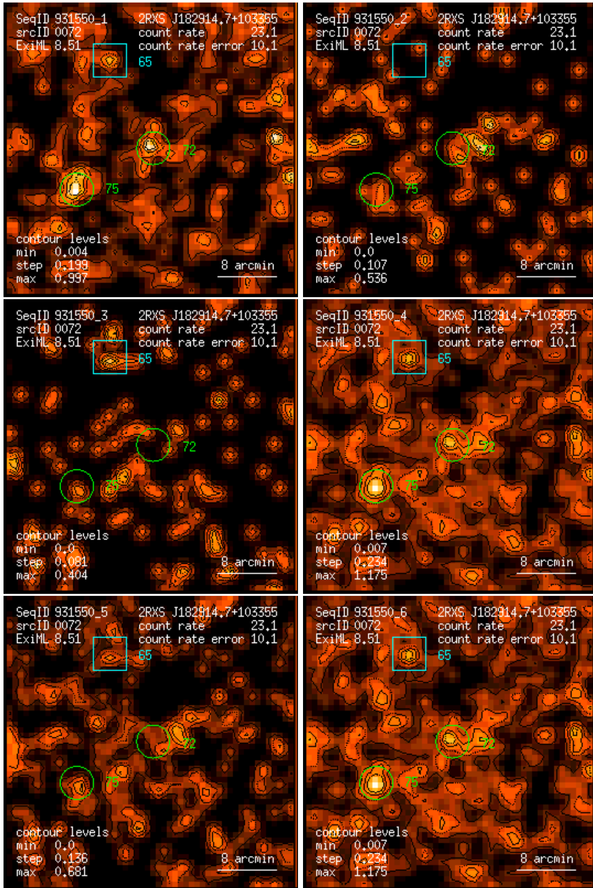
Figure 72: RASS 931550: detection 0072: band rate images, Gaussian filter: (1) PSPC channels 11 – 41, (2) 52 – 90, (3) 91 – 201, (4) 11 – 235, (5) 52 – 201, (6) 11 – 201. Broad band rates in counts/ks. Band rate contour levels in counts/ks/arcmin 2 .
