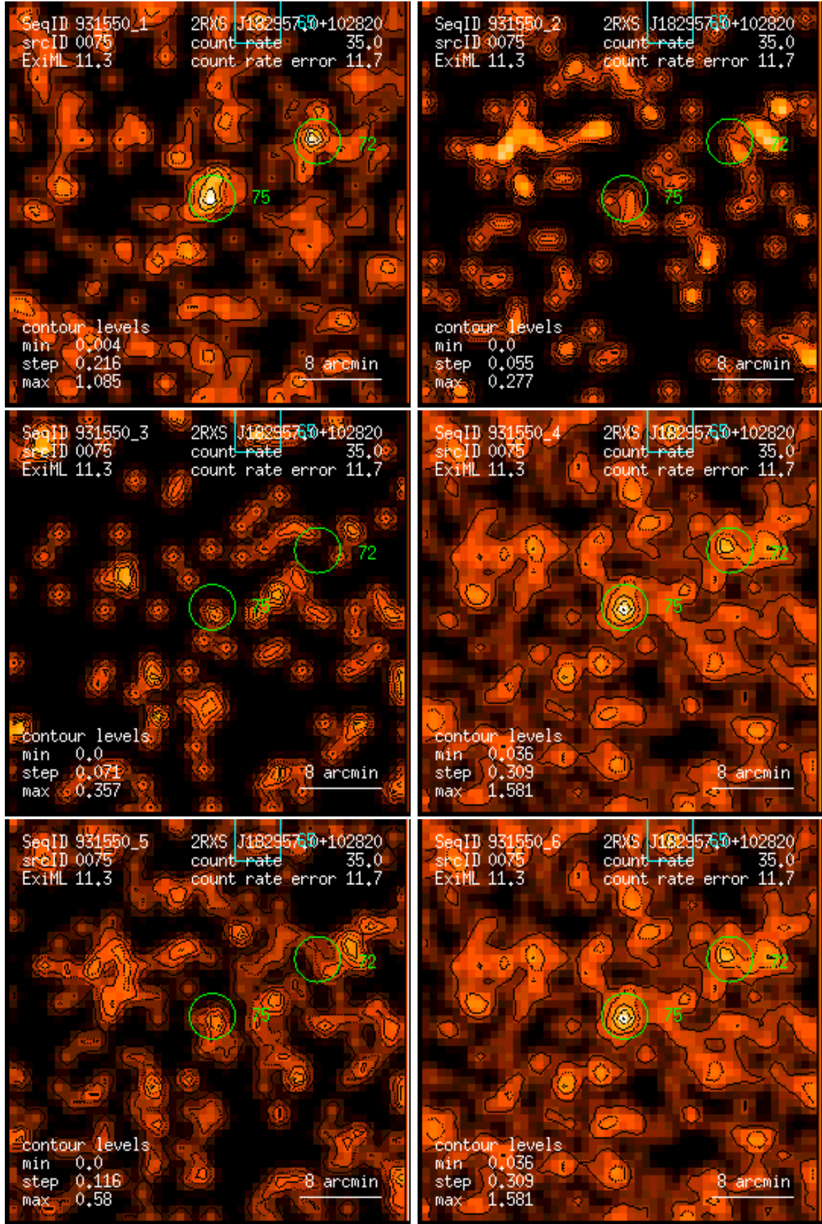
Figure 75: RASS 931550: detection 0075: band rate images, Gaussian filter: (1) PSPC channels 11 – 41, (2) 52 – 90, (3) 91 – 201, (4) 11 – 235, (5) 52 – 201, (6) 11 – 201. Broad band rates in counts/ks. Band rate contour levels in counts/ks/arcmin 2 .
