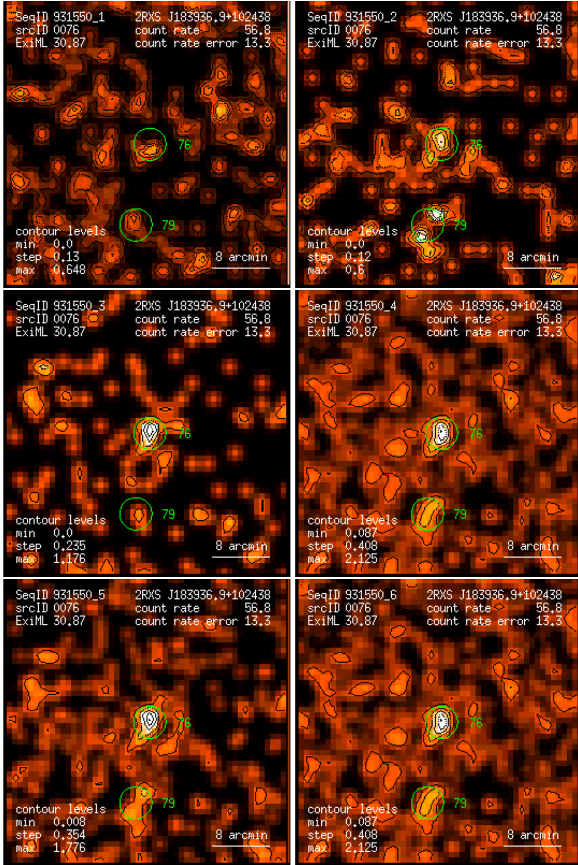
Figure 76: RASS 931550: detection 0076: band rate images, Gaussian filter: (1) PSPC channels 11 – 41, (2) 52 – 90, (3) 91 – 201, (4) 11 – 235, (5) 52 – 201, (6) 11 – 201. Broad band rates in counts/ks. Band rate contour levels in counts/ks/arcmin 2 .
