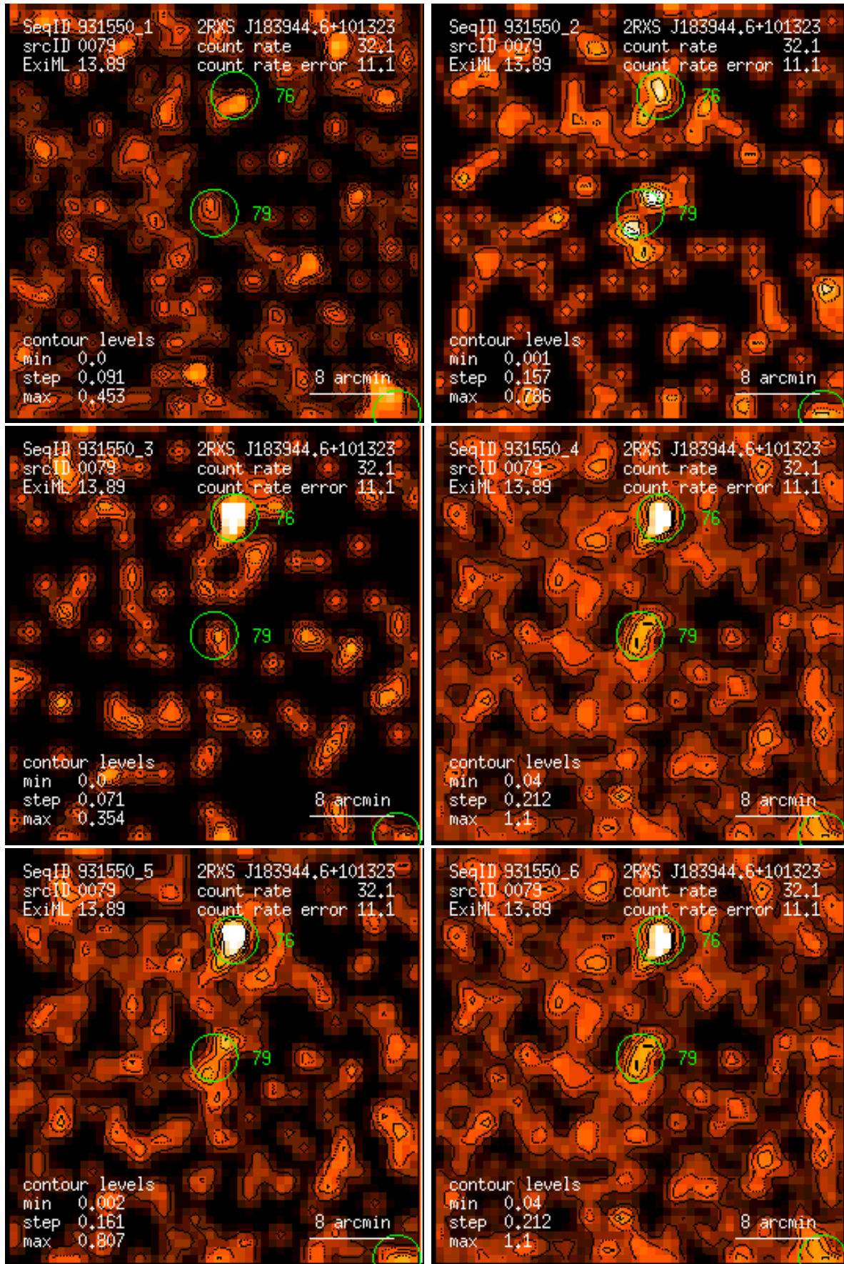
Figure 79: RASS 931550: detection 0079: band rate images, Gaussian filter: (1) PSPC channels 11 – 41, (2) 52 – 90, (3) 91 – 201, (4) 11 – 235, (5) 52 – 201, (6) 11 – 201. Broad band rates in counts/ks. Band rate contour levels in counts/ks/arcmin 2 .
