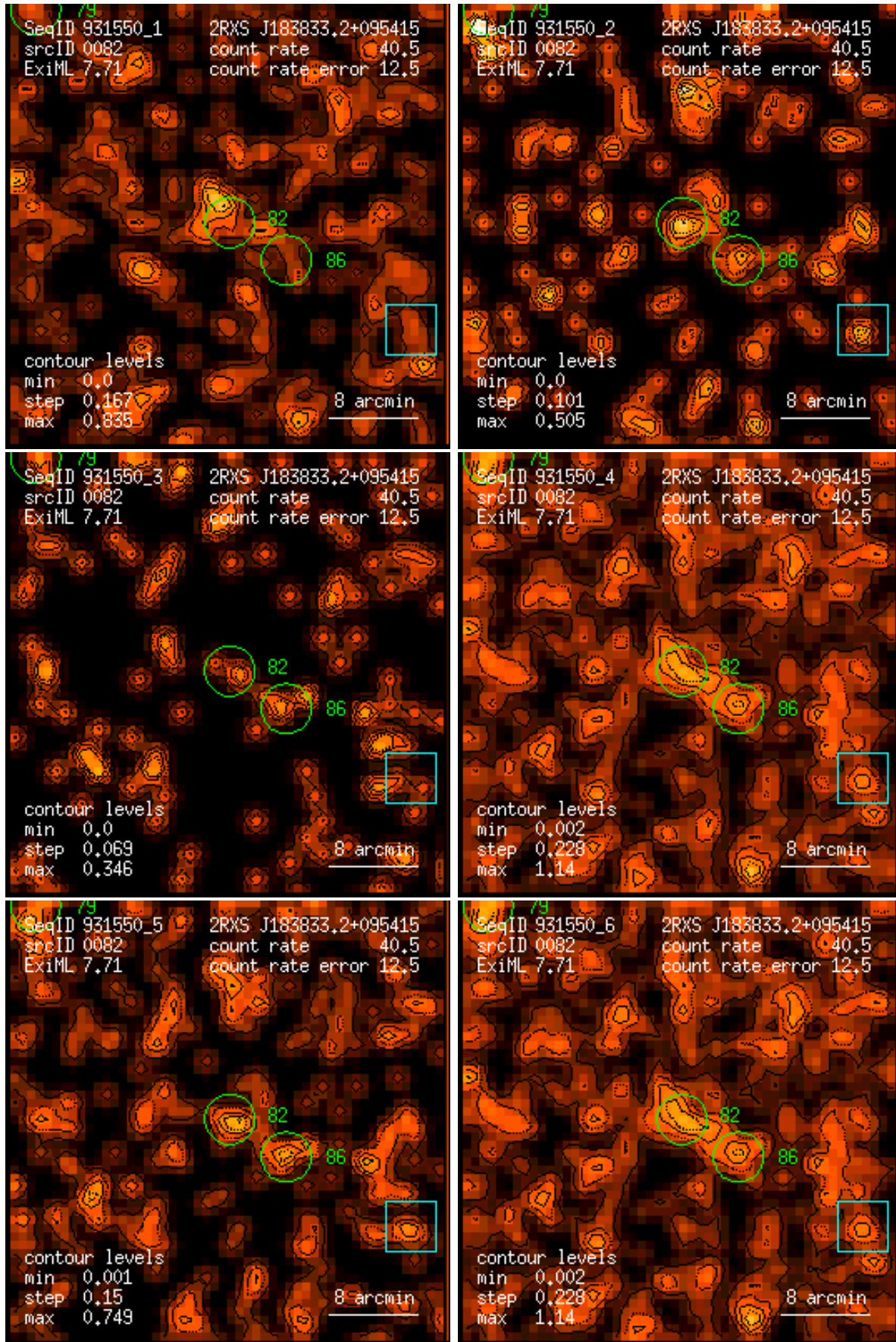
Figure 82: RASS 931550: detection 0082: band rate images, Gaussian filter: (1) PSPC channels 11 – 41, (2) 52 – 90, (3) 91 – 201, (4) 11 – 235, (5) 52 – 201, (6) 11 – 201. Broad band rates in counts/ks. Band rate contour levels in counts/ks/arcmin 2 .
