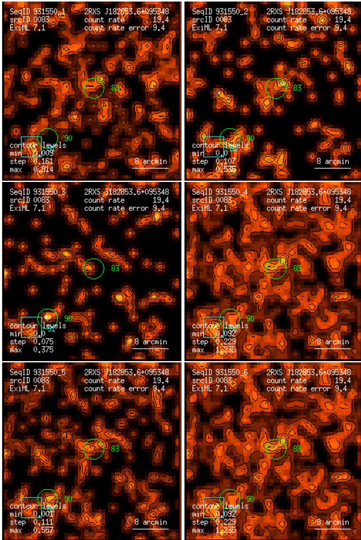
Figure 83: RASS 931550: detection 0083: band rate images, Gaussian filter: (1) PSPC channels 11 – 41, (2) 52 – 90, (3) 91 – 201, (4) 11 – 235, (5) 52 – 201, (6) 11 – 201. Broad band rates in counts/ks. Band rate contour levels in counts/ks/arcmin 2 .
