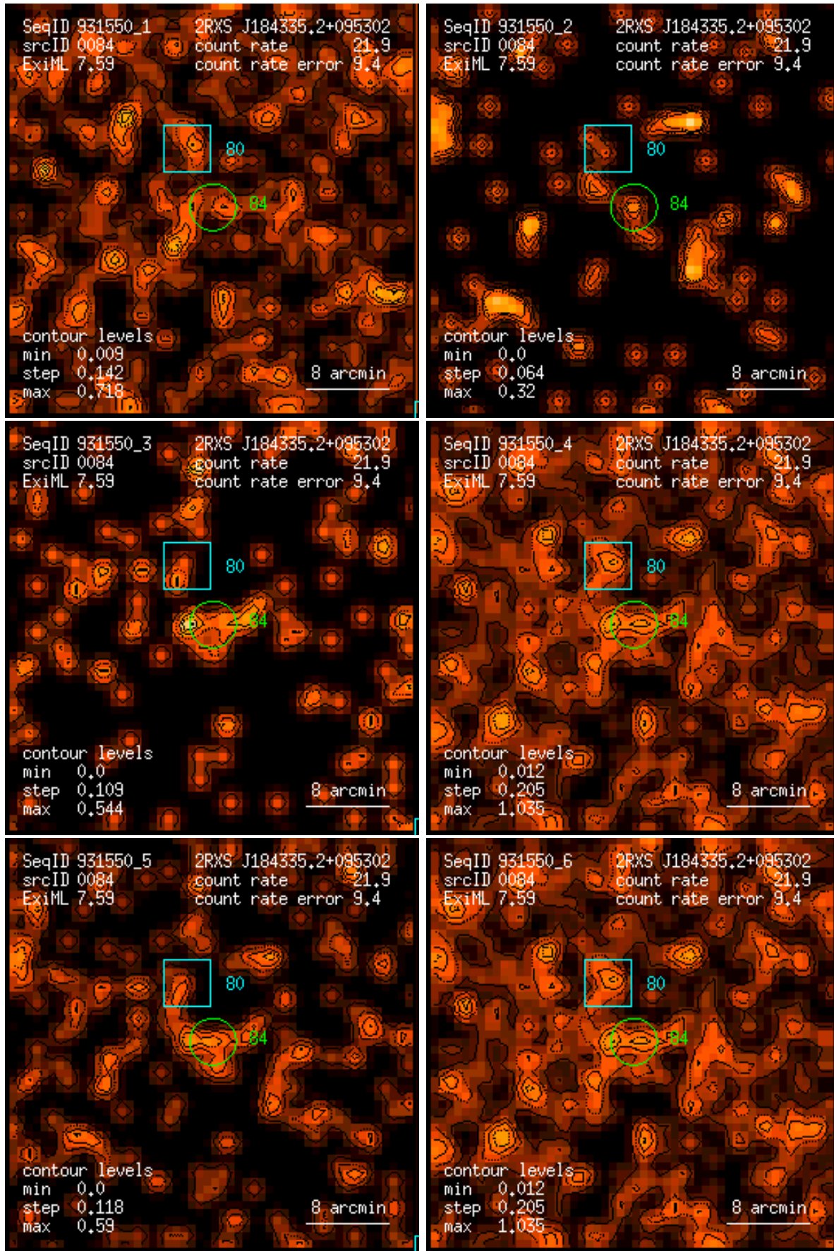
Figure 84: RASS 931550: detection 0084: band rate images, Gaussian filter: (1) PSPC channels 11 – 41, (2) 52 – 90, (3) 91 – 201, (4) 11 – 235, (5) 52 – 201, (6) 11 – 201. Broad band rates in counts/ks. Band rate contour levels in counts/ks/arcmin 2 .
