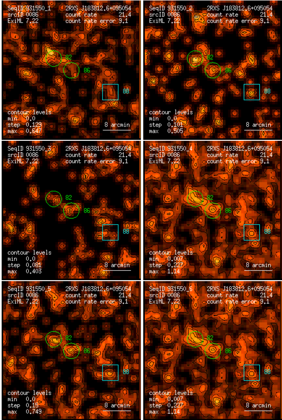
Figure 86: RASS 931550: detection 0086: band rate images, Gaussian filter: (1) PSPC channels 11 – 41, (2) 52 – 90, (3) 91 – 201, (4) 11 – 235, (5) 52 – 201, (6) 11 – 201. Broad band rates in counts/ks. Band rate contour levels in counts/ks/arcmin 2 .
