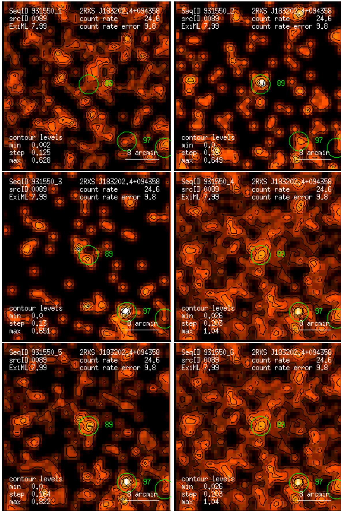
Figure 89: RASS 931550: detection 0089: band rate images, Gaussian filter: (1) PSPC channels 11 – 41, (2) 52 – 90, (3) 91 – 201, (4) 11 – 235, (5) 52 – 201, (6) 11 – 201. Broad band rates in counts/ks. Band rate contour levels in counts/ks/arcmin 2 .
