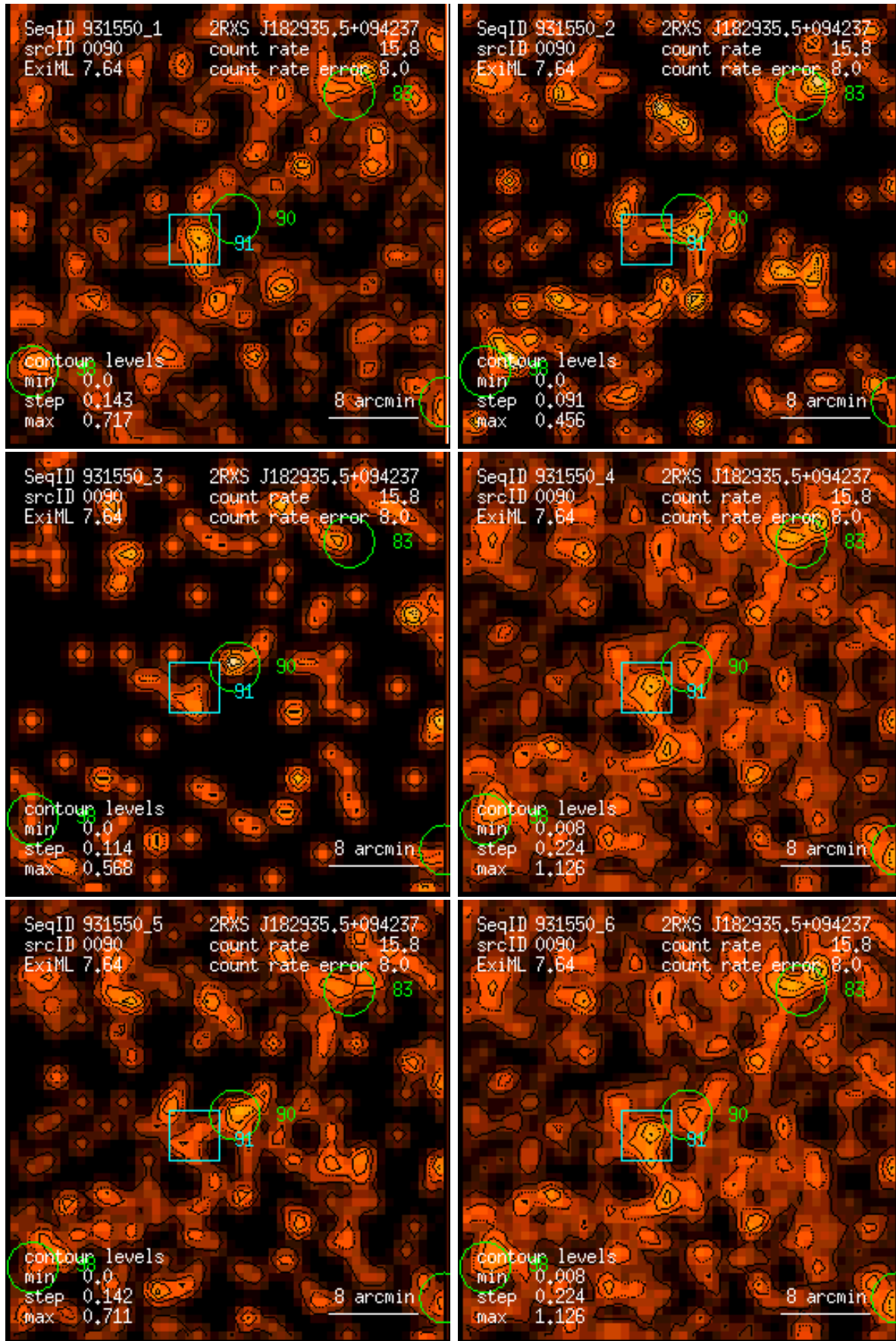
Figure 90: RASS 931550: detection 0090: band rate images, Gaussian filter: (1) PSPC channels 11 – 41, (2) 52 – 90, (3) 91 – 201, (4) 11 – 235, (5) 52 – 201, (6) 11 – 201. Broad band rates in counts/ks. Band rate contour levels in counts/ks/arcmin 2 .
