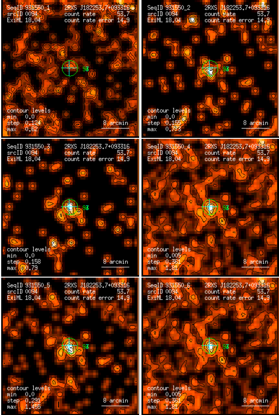
Figure 94: RASS 931550: detection 0094: band rate images, Gaussian filter: (1) PSPC channels 11 – 41, (2) 52 – 90, (3) 91 – 201, (4) 11 – 235, (5) 52 – 201, (6) 11 – 201. Broad band rates in counts/ks. Band rate contour levels in counts/ks/arcmin 2 .
