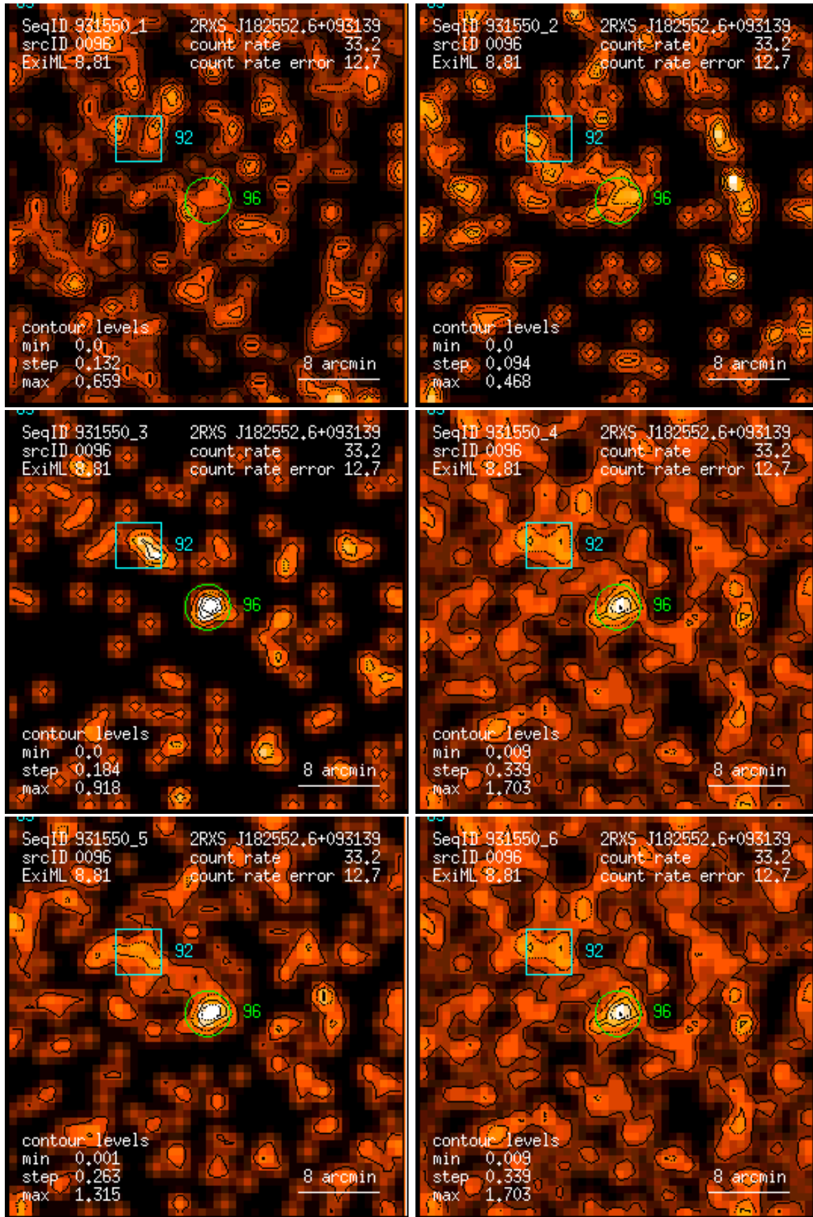
Figure 96: RASS 931550: detection 0096: band rate images, Gaussian filter: (1) PSPC channels 11 – 41, (2) 52 – 90, (3) 91 – 201, (4) 11 – 235, (5) 52 – 201, (6) 11 – 201. Broad band rates in counts/ks. Band rate contour levels in counts/ks/arcmin 2 .
