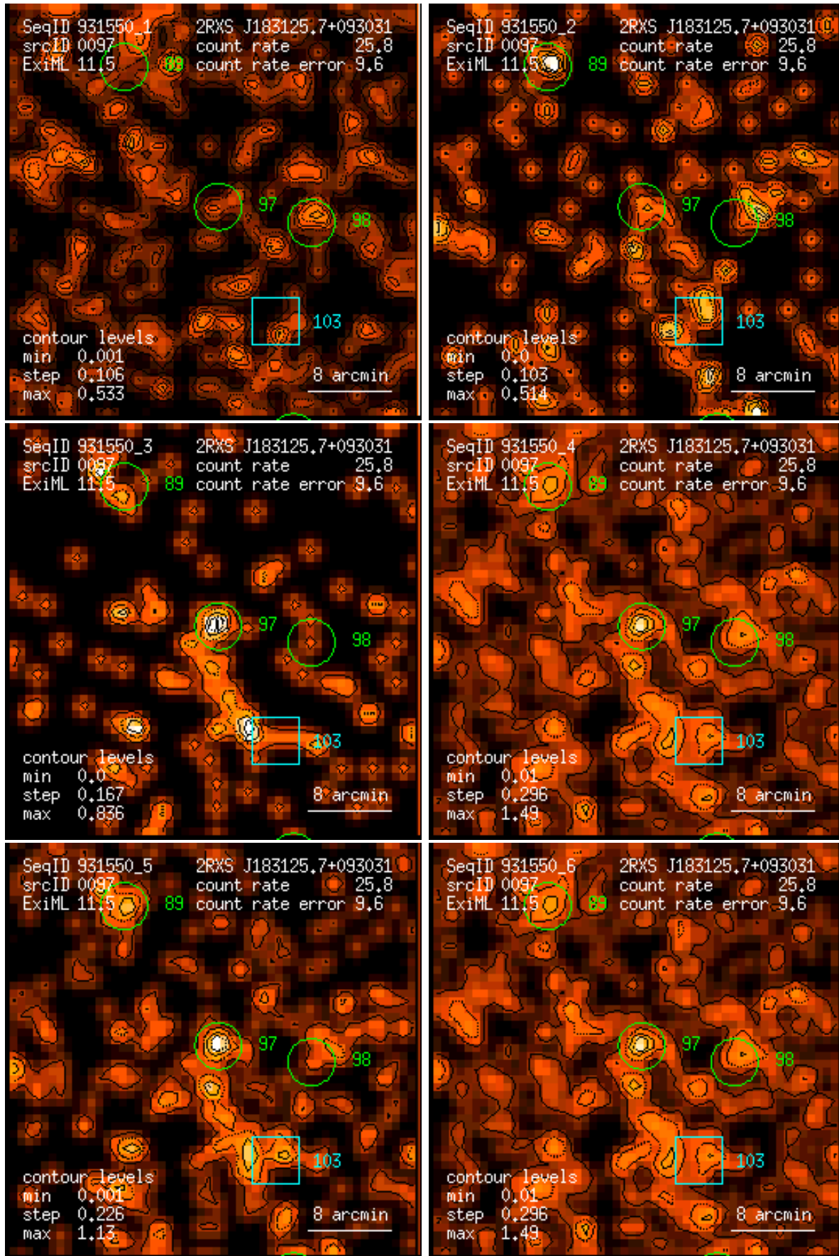
Figure 97: RASS 931550: detection 0097: band rate images, Gaussian filter: (1) PSPC channels 11 – 41, (2) 52 – 90, (3) 91 – 201, (4) 11 – 235, (5) 52 – 201, (6) 11 – 201. Broad band rates in counts/ks. Band rate contour levels in counts/ks/arcmin 2 .
