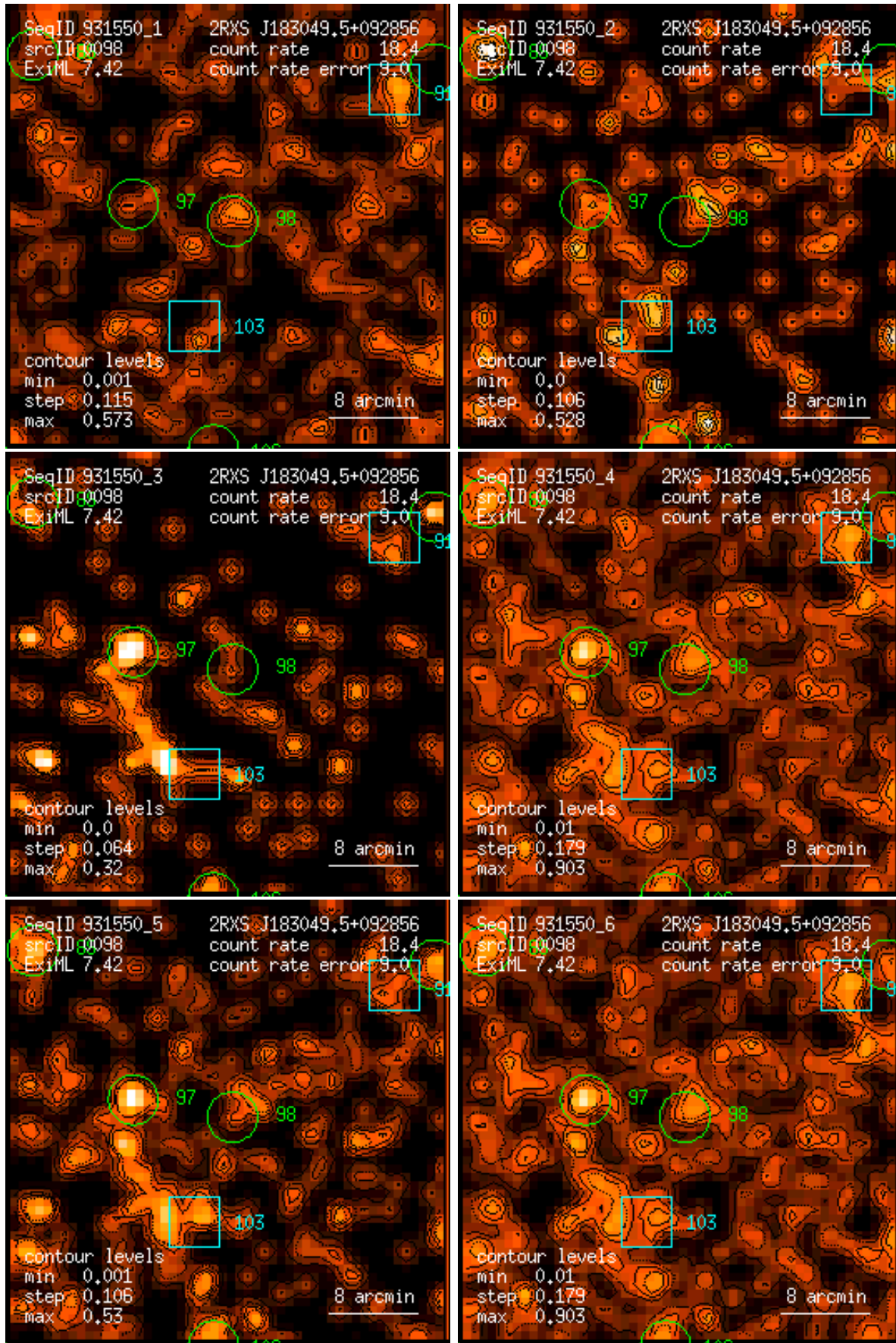
Figure 98: RASS 931550: detection 0098: band rate images, Gaussian filter: (1) PSPC channels 11 – 41, (2) 52 – 90, (3) 91 – 201, (4) 11 – 235, (5) 52 – 201, (6) 11 – 201. Broad band rates in counts/ks. Band rate contour levels in counts/ks/arcmin 2 .
