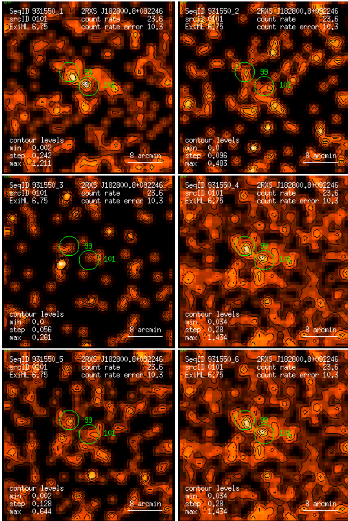
Figure 101: RASS 931550: detection 0101: band rate images, Gaussian filter: (1) PSPC channels 11 – 41, (2) 52 – 90, (3) 91 – 201, (4) 11 – 235, (5) 52 – 201, (6) 11 – 201. Broad band rates in counts/ks. Band rate contour levels in counts/ks/arcmin 2 .
