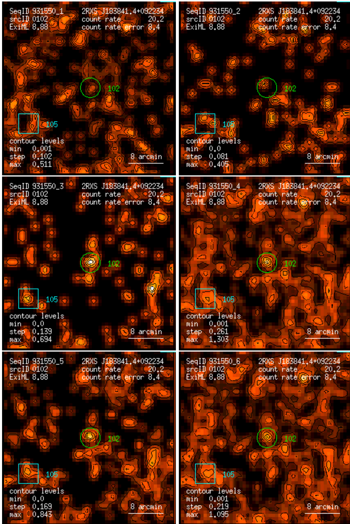
Figure 102: RASS 931550: detection 0102: band rate images, Gaussian filter: (1) PSPC channels 11 – 41, (2) 52 – 90, (3) 91 – 201, (4) 11 – 235, (5) 52 – 201, (6) 11 – 201. Broad band rates in counts/ks. Band rate contour levels in counts/ks/arcmin 2 .
