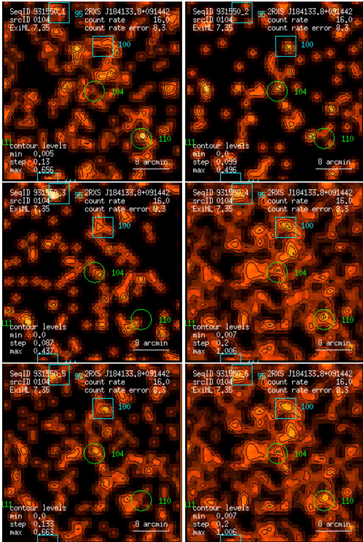
Figure 104: RASS 931550: detection 0104: band rate images, Gaussian filter: (1) PSPC channels 11 – 41, (2) 52 – 90, (3) 91 – 201, (4) 11 – 235, (5) 52 – 201, (6) 11 – 201. Broad band rates in counts/ks. Band rate contour levels in counts/ks/arcmin 2 .
