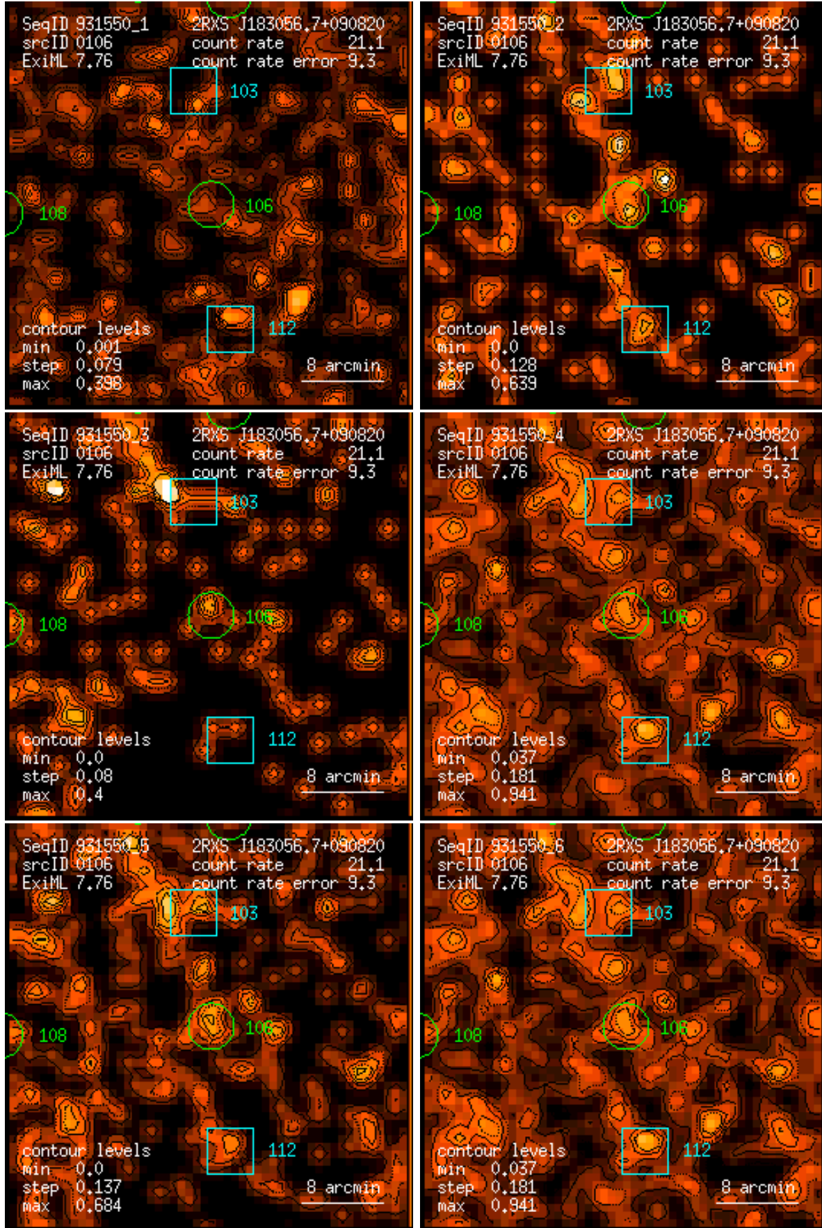
Figure 106: RASS 931550: detection 0106: band rate images, Gaussian filter: (1) PSPC channels 11 – 41, (2) 52 – 90, (3) 91 – 201, (4) 11 – 235, (5) 52 – 201, (6) 11 – 201. Broad band rates in counts/ks. Band rate contour levels in counts/ks/arcmin 2 .
