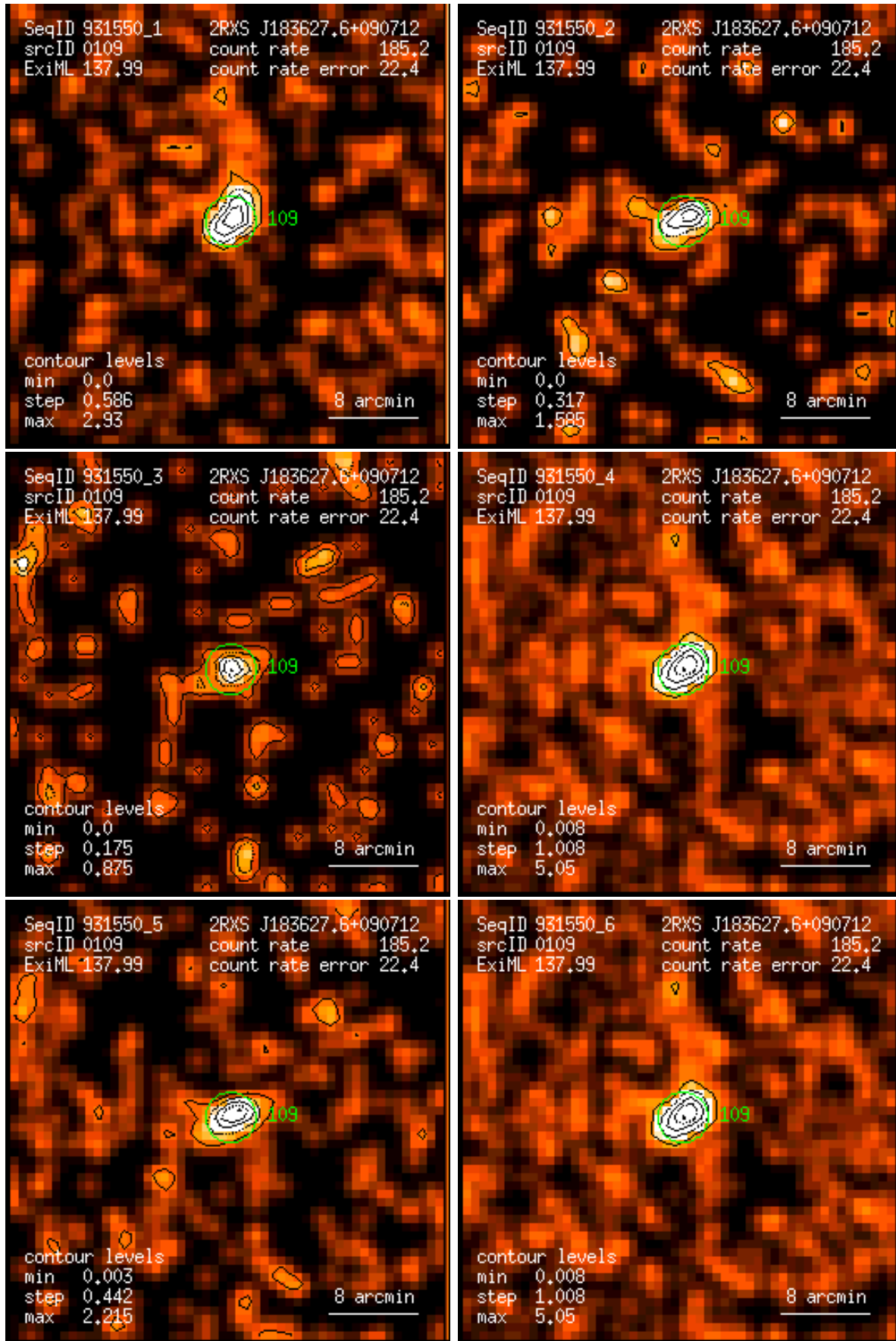
Figure 109: RASS 931550: detection 0109: band rate images, Gaussian filter: (1) PSPC channels 11 – 41, (2) 52 – 90, (3) 91 – 201, (4) 11 – 235, (5) 52 – 201, (6) 11 – 201. Broad band rates in counts/ks. Band rate contour levels in counts/ks/arcmin 2 .
