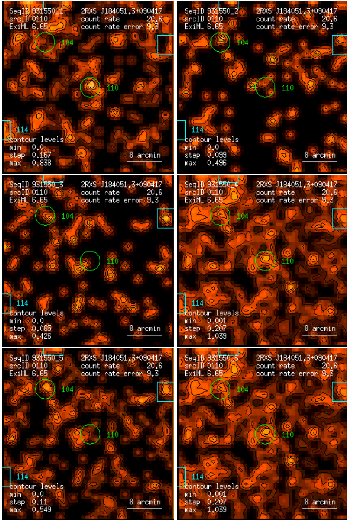
Figure 110: RASS 931550: detection 0110: band rate images, Gaussian filter: (1) PSPC channels 11 – 41, (2) 52 – 90, (3) 91 – 201, (4) 11 – 235, (5) 52 – 201, (6) 11 – 201. Broad band rates in counts/ks. Band rate contour levels in counts/ks/arcmin 2 .
