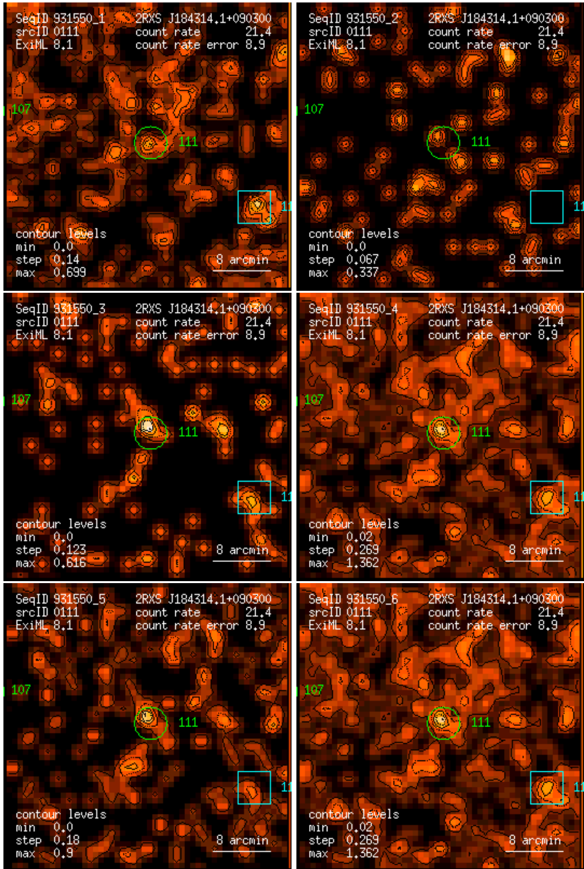
Figure 111: RASS 931550: detection 0111: band rate images, Gaussian filter: (1) PSPC channels 11 – 41, (2) 52 – 90, (3) 91 – 201, (4) 11 – 235, (5) 52 – 201, (6) 11 – 201. Broad band rates in counts/ks. Band rate contour levels in counts/ks/arcmin 2 .
