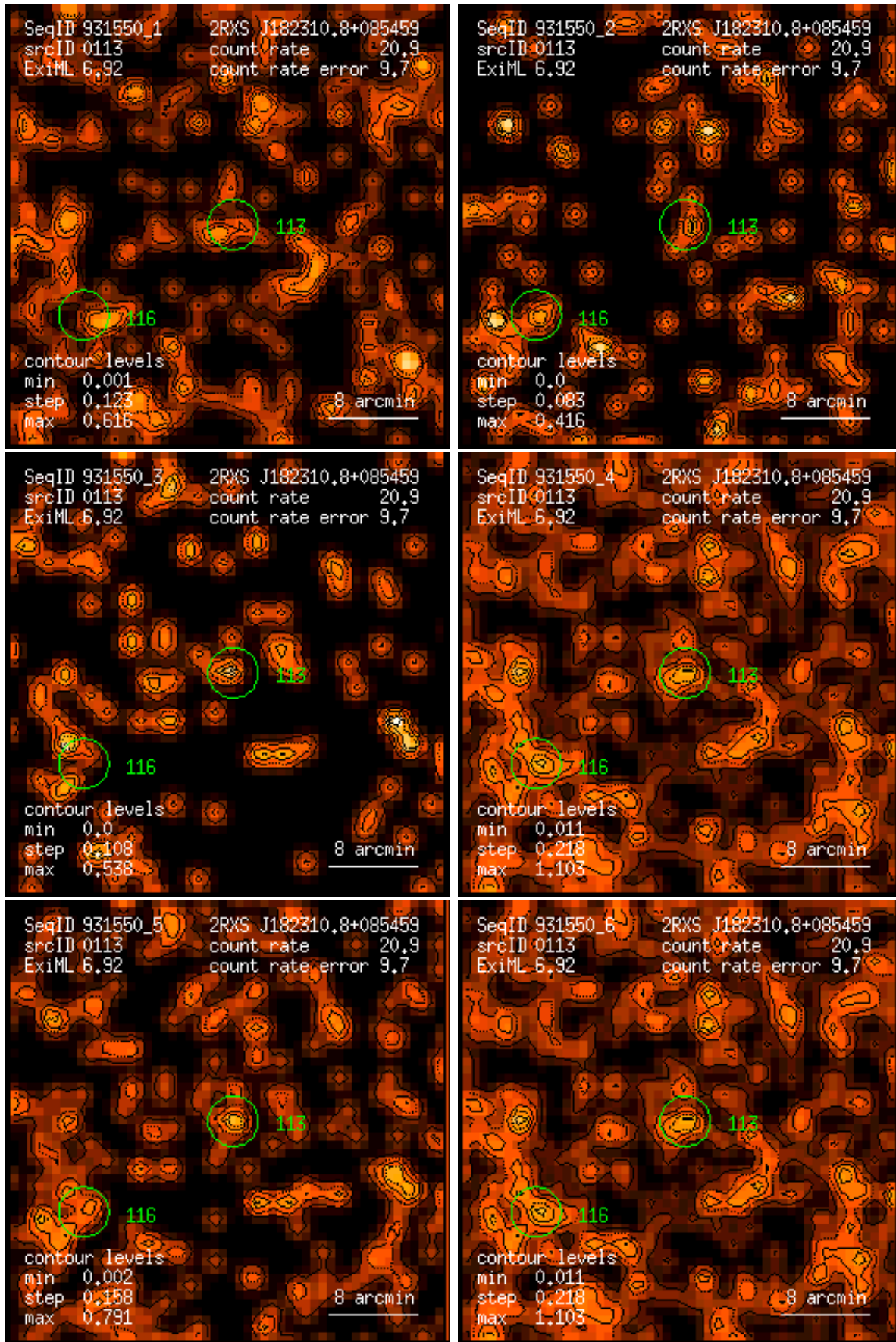
Figure 113: RASS 931550: detection 0113: band rate images, Gaussian filter: (1) PSPC channels 11 – 41, (2) 52 – 90, (3) 91 – 201, (4) 11 – 235, (5) 52 – 201, (6) 11 – 201. Broad band rates in counts/ks. Band rate contour levels in counts/ks/arcmin 2 .
