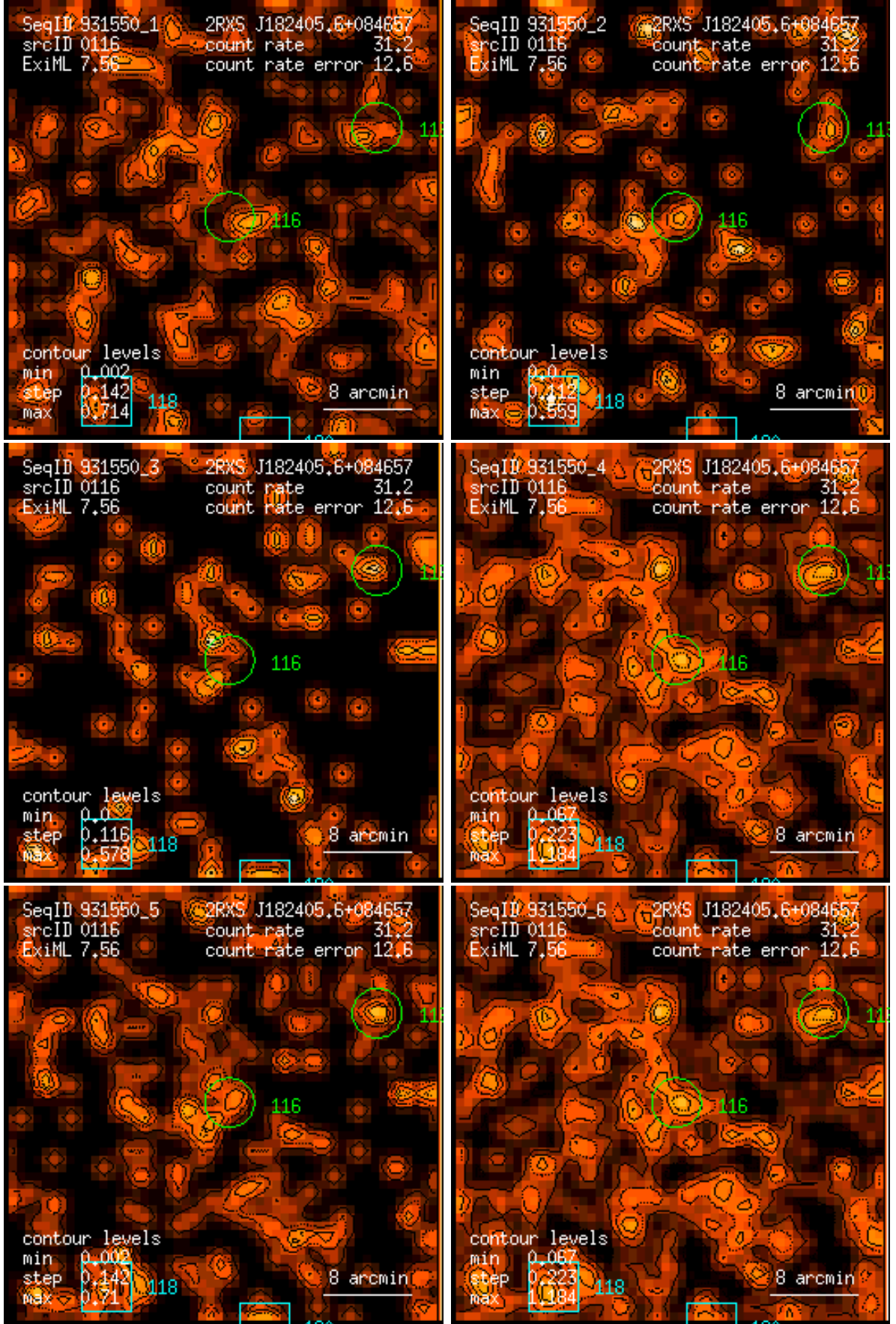
Figure 116: RASS 931550: detection 0116: band rate images, Gaussian filter: (1) PSPC channels 11 – 41, (2) 52 – 90, (3) 91 – 201, (4) 11 – 235, (5) 52 – 201, (6) 11 – 201. Broad band rates in counts/ks. Band rate contour levels in counts/ks/arcmin 2 .
