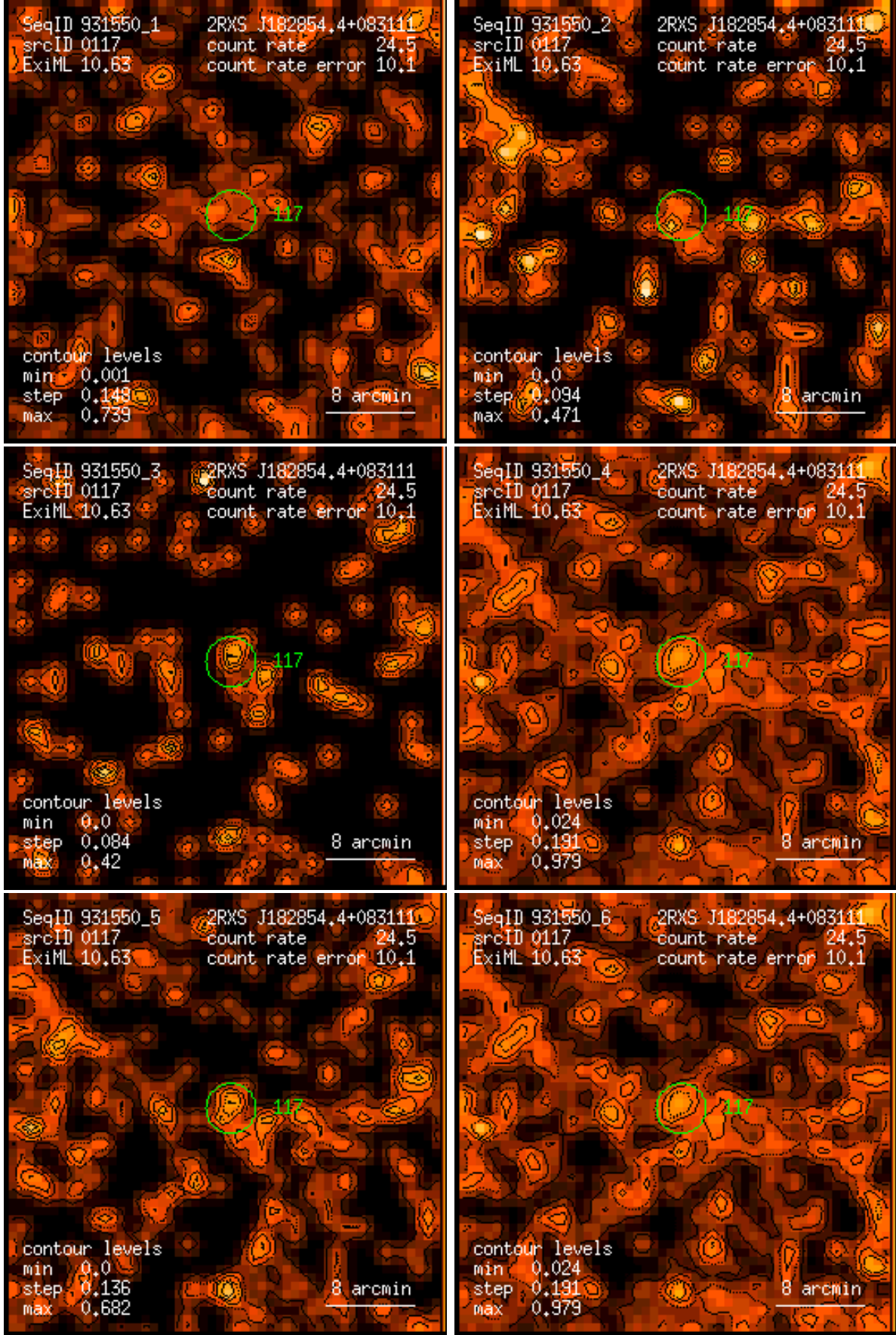
Figure 117: RASS 931550: detection 0117: band rate images, Gaussian filter: (1) PSPC channels 11 – 41, (2) 52 – 90, (3) 91 – 201, (4) 11 – 235, (5) 52 – 201, (6) 11 – 201. Broad band rates in counts/ks. Band rate contour levels in counts/ks/arcmin 2 .
