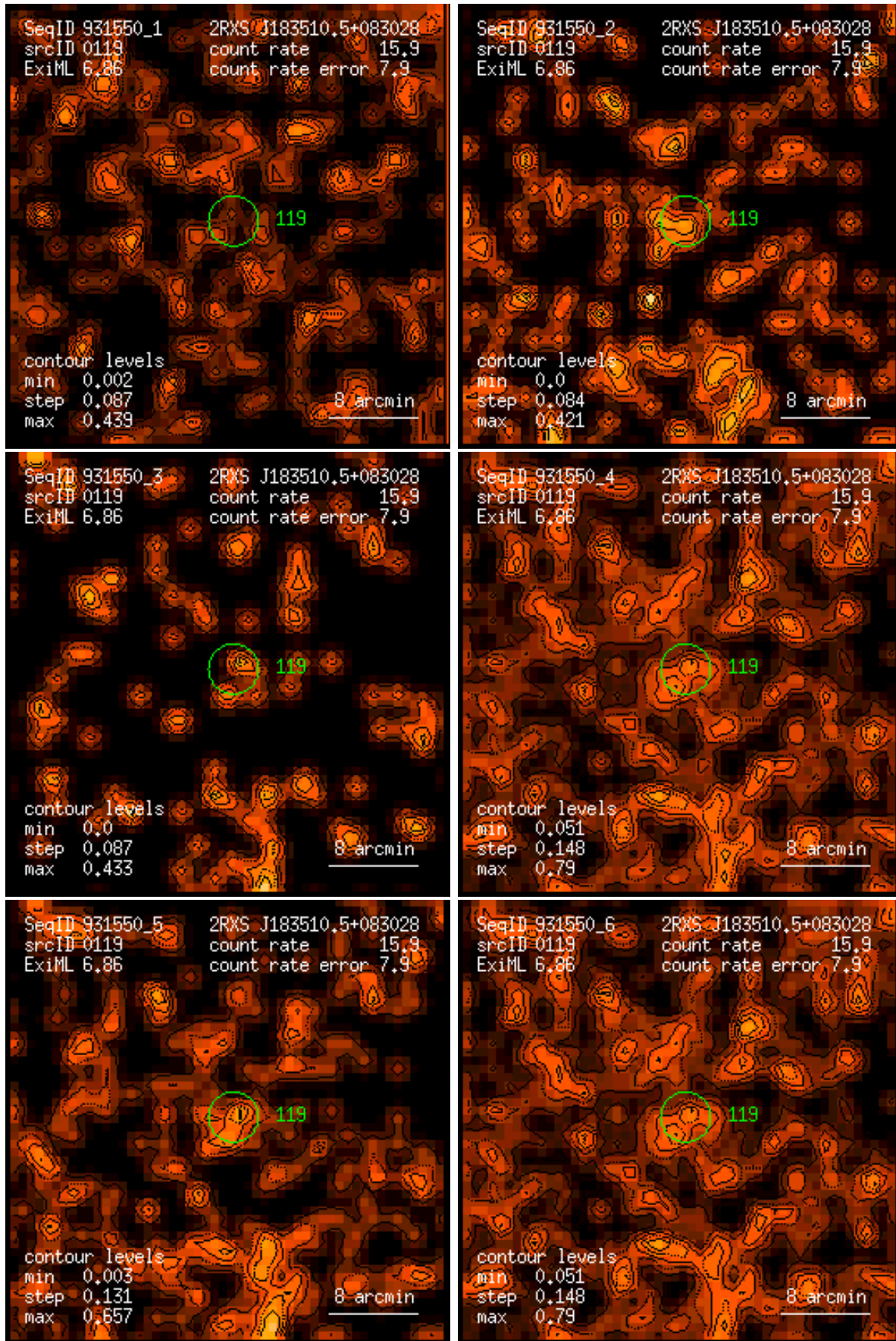
Figure 119: RASS 931550: detection 0119: band rate images, Gaussian filter: (1) PSPC channels 11 – 41, (2) 52 – 90, (3) 91 – 201, (4) 11 – 235, (5) 52 – 201, (6) 11 – 201. Broad band rates in counts/ks. Band rate contour levels in counts/ks/arcmin 2 .
