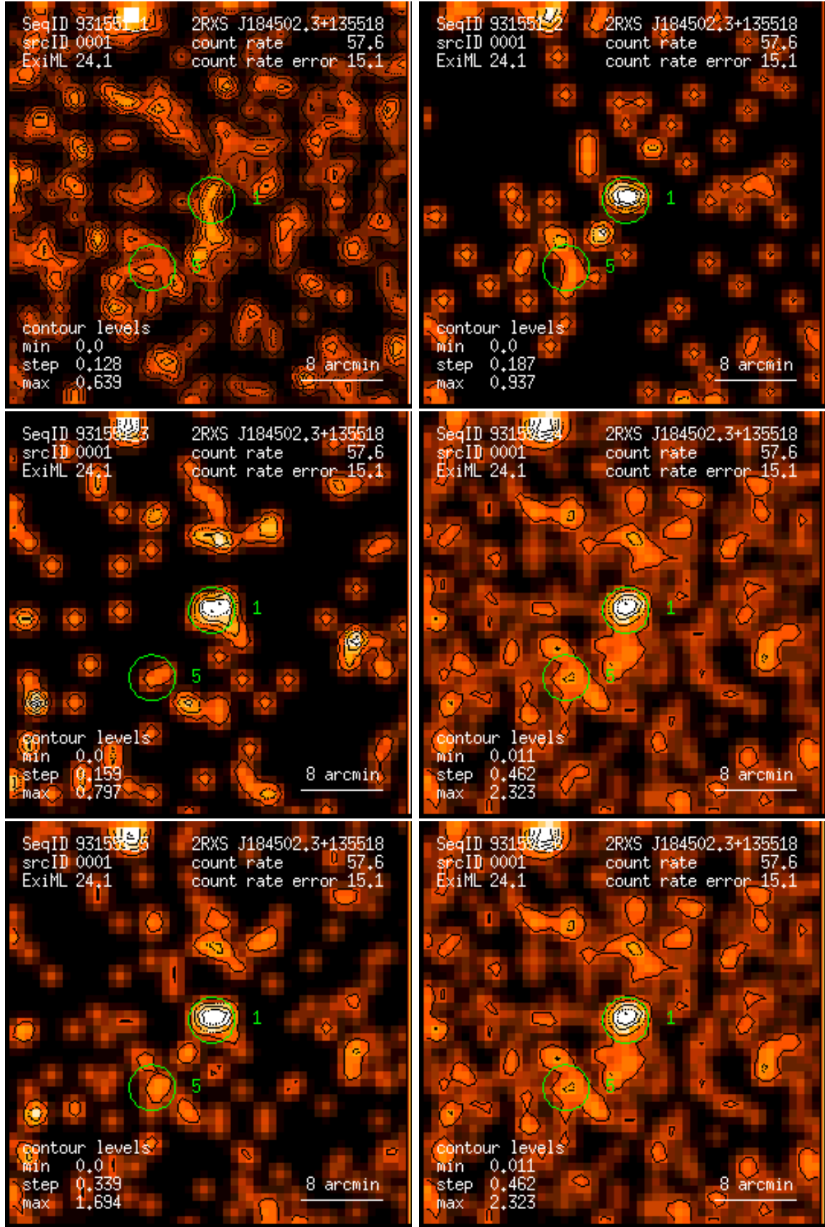
Figure 1: RASS 931551: detection 0001: band rate images, Gaussian filter: (1) PSPC channels 11 – 41, (2) 52 – 90, (3) 91 – 201, (4) 11 – 235, (5) 52 – 201, (6) 11 – 201. Broad band rates in counts/ks. Band rate contour levels in counts/ks/arcmin 2 .
